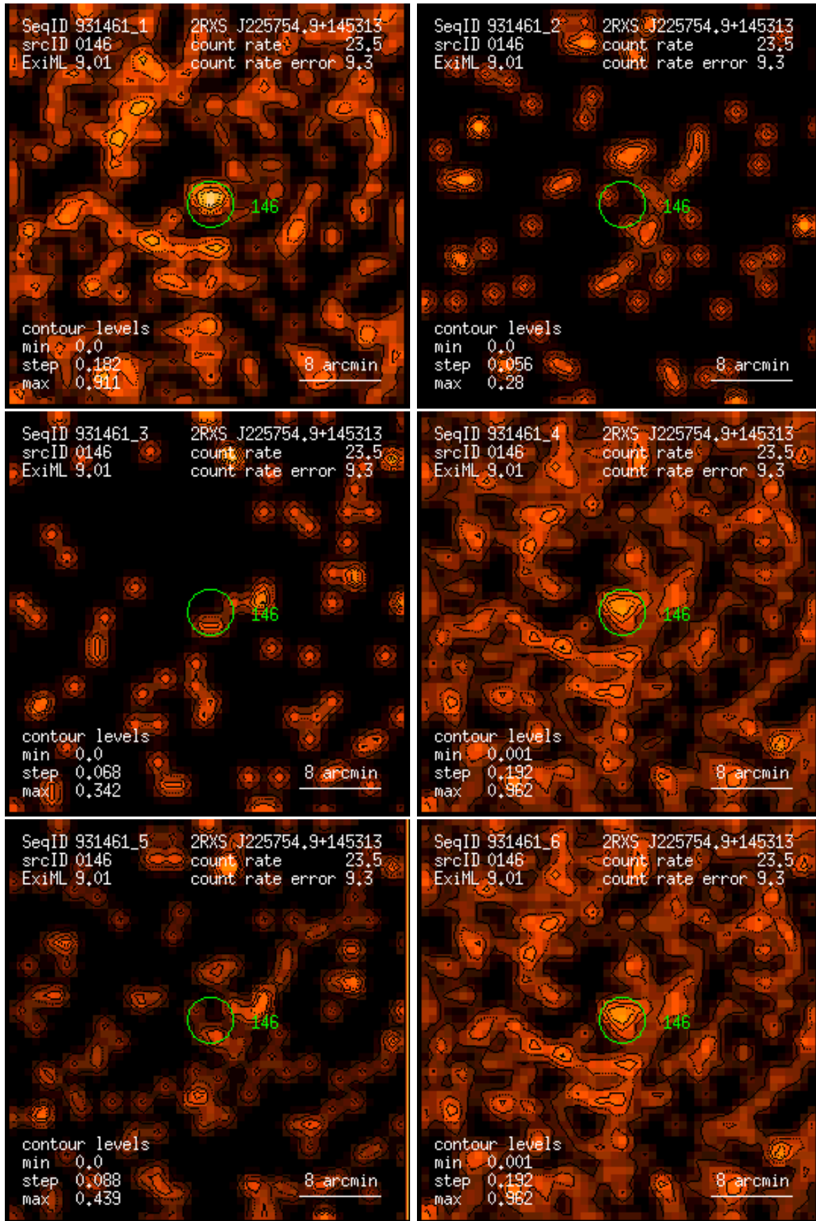
Figure 146: RASS 931461: detection 0146: band rate images, Gaussian filter: (1) PSPC channels 11 – 41, (2) 52 – 90, (3) 91 – 201, (4) 11 – 235, (5) 52 – 201, (6) 11 – 201. Broad band rates in counts/ks. Band rate contour levels in counts/ks/arcmin 2 .
