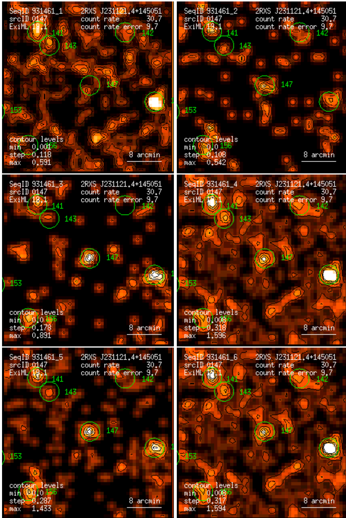
Figure 147: RASS 931461: detection 0147: band rate images, Gaussian filter: (1) PSPC channels 11 – 41, (2) 52 – 90, (3) 91 – 201, (4) 11 – 235, (5) 52 – 201, (6) 11 – 201. Broad band rates in counts/ks. Band rate contour levels in counts/ks/arcmin 2 .
