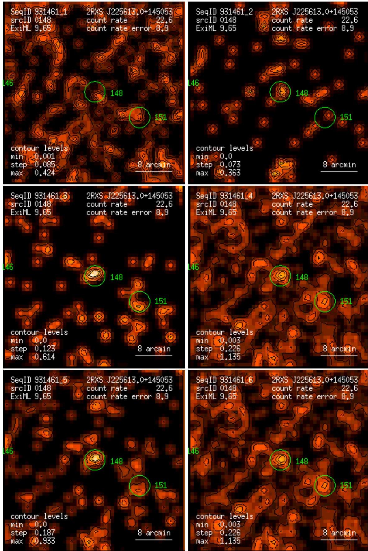
Figure 148: RASS 931461: detection 0148: band rate images, Gaussian filter: (1) PSPC channels 11 – 41, (2) 52 – 90, (3) 91 – 201, (4) 11 – 235, (5) 52 – 201, (6) 11 – 201. Broad band rates in counts/ks. Band rate contour levels in counts/ks/arcmin 2 .
