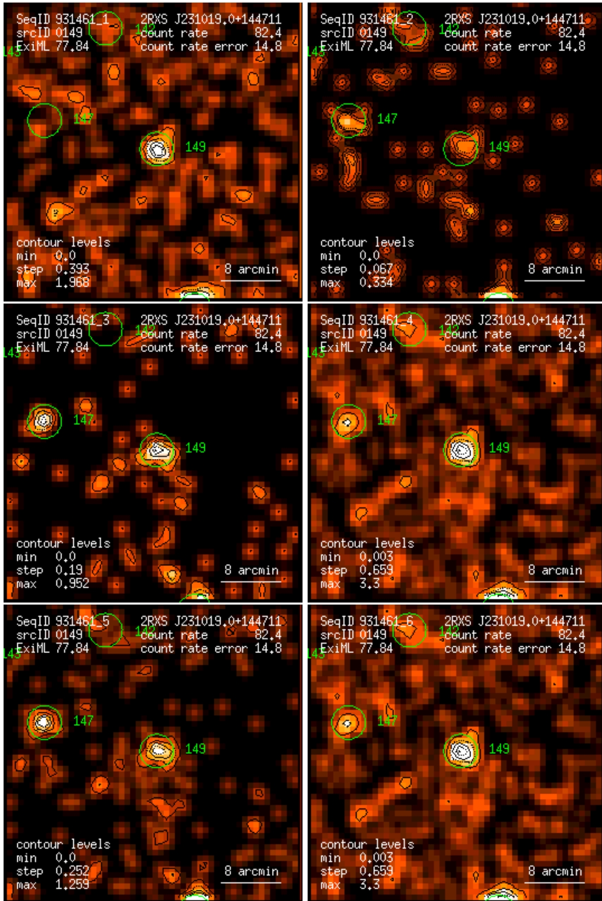
Figure 149: RASS 931461: detection 0149: band rate images, Gaussian filter: (1) PSPC channels 11 – 41, (2) 52 – 90, (3) 91 – 201, (4) 11 – 235, (5) 52 – 201, (6) 11 – 201. Broad band rates in counts/ks. Band rate contour levels in counts/ks/arcmin 2 .
