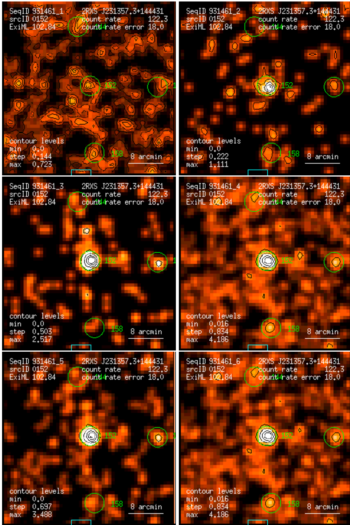
Figure 152: RASS 931461: detection 0152: band rate images, Gaussian filter: (1) PSPC channels 11 – 41, (2) 52 – 90, (3) 91 – 201, (4) 11 – 235, (5) 52 – 201, (6) 11 – 201. Broad band rates in counts/ks. Band rate contour levels in counts/ks/arcmin 2 .
