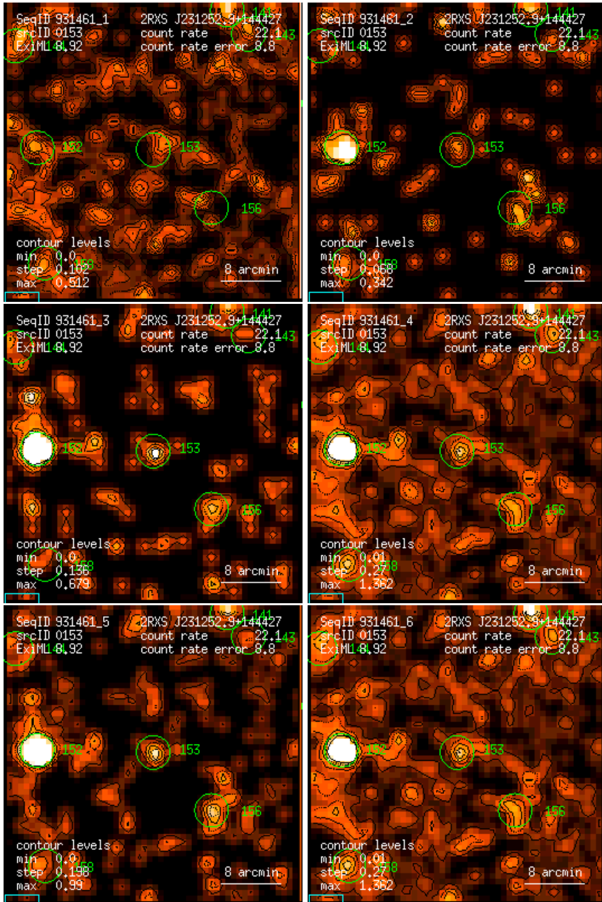
Figure 153: RASS 931461: detection 0153: band rate images, Gaussian filter: (1) PSPC channels 11 – 41, (2) 52 – 90, (3) 91 – 201, (4) 11 – 235, (5) 52 – 201, (6) 11 – 201. Broad band rates in counts/ks. Band rate contour levels in counts/ks/arcmin 2 .
