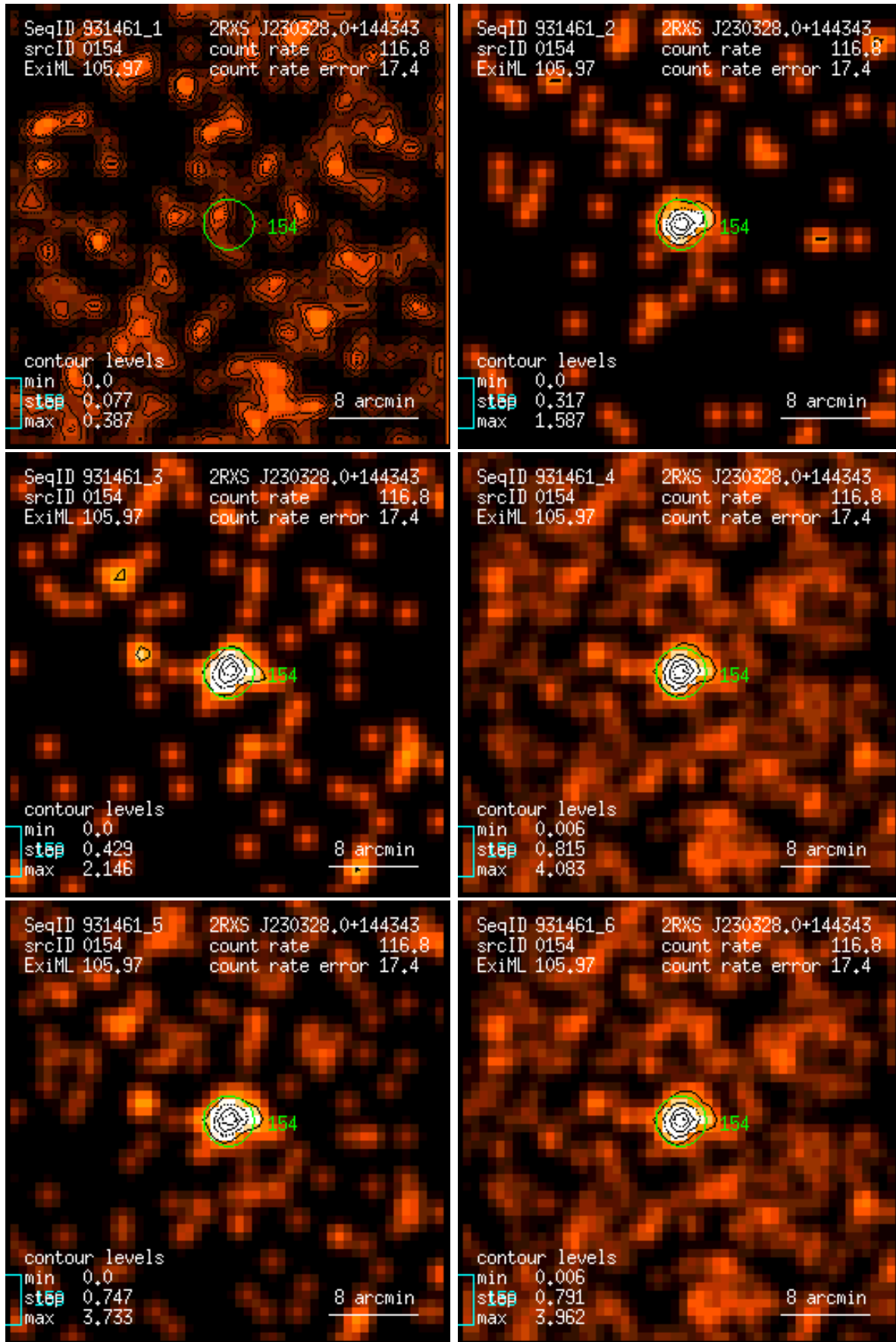
Figure 154: RASS 931461: detection 0154: band rate images, Gaussian filter: (1) PSPC channels 11 – 41, (2) 52 – 90, (3) 91 – 201, (4) 11 – 235, (5) 52 – 201, (6) 11 – 201. Broad band rates in counts/ks. Band rate contour levels in counts/ks/arcmin 2 .
