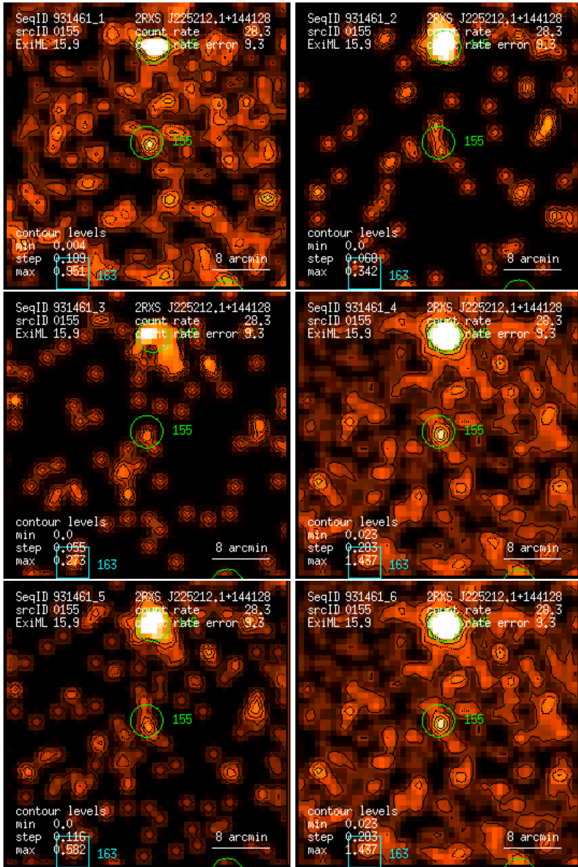
Figure 155: RASS 931461: detection 0155: band rate images, Gaussian filter: (1) PSPC channels 11 – 41, (2) 52 – 90, (3) 91 – 201, (4) 11 – 235, (5) 52 – 201, (6) 11 – 201. Broad band rates in counts/ks. Band rate contour levels in counts/ks/arcmin 2 .
