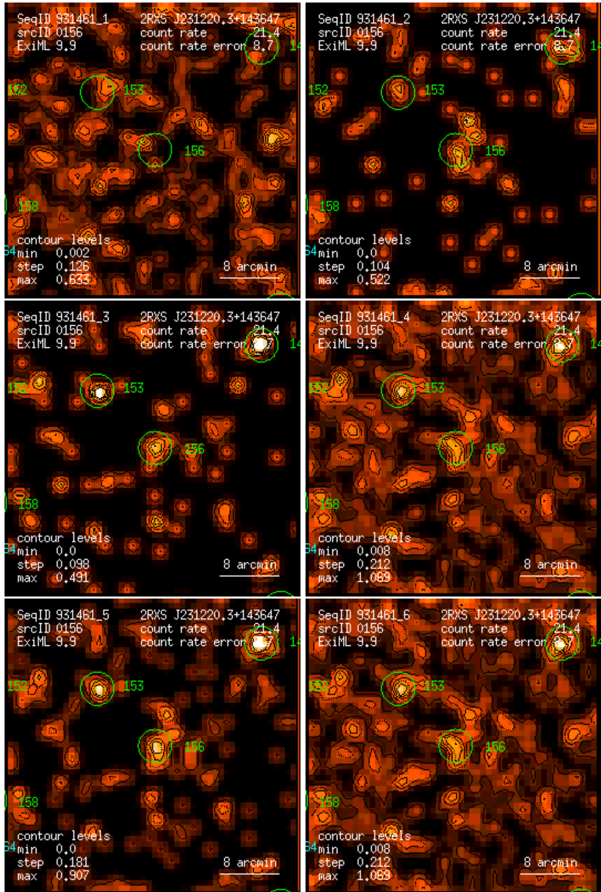
Figure 156: RASS 931461: detection 0156: band rate images, Gaussian filter: (1) PSPC channels 11 – 41, (2) 52 – 90, (3) 91 – 201, (4) 11 – 235, (5) 52 – 201, (6) 11 – 201. Broad band rates in counts/ks. Band rate contour levels in counts/ks/arcmin 2 .
