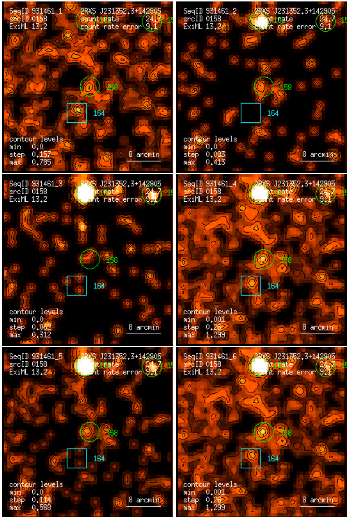
Figure 158: RASS 931461: detection 0158: band rate images, Gaussian filter: (1) PSPC channels 11 – 41, (2) 52 – 90, (3) 91 – 201, (4) 11 – 235, (5) 52 – 201, (6) 11 – 201. Broad band rates in counts/ks. Band rate contour levels in counts/ks/arcmin 2 .
