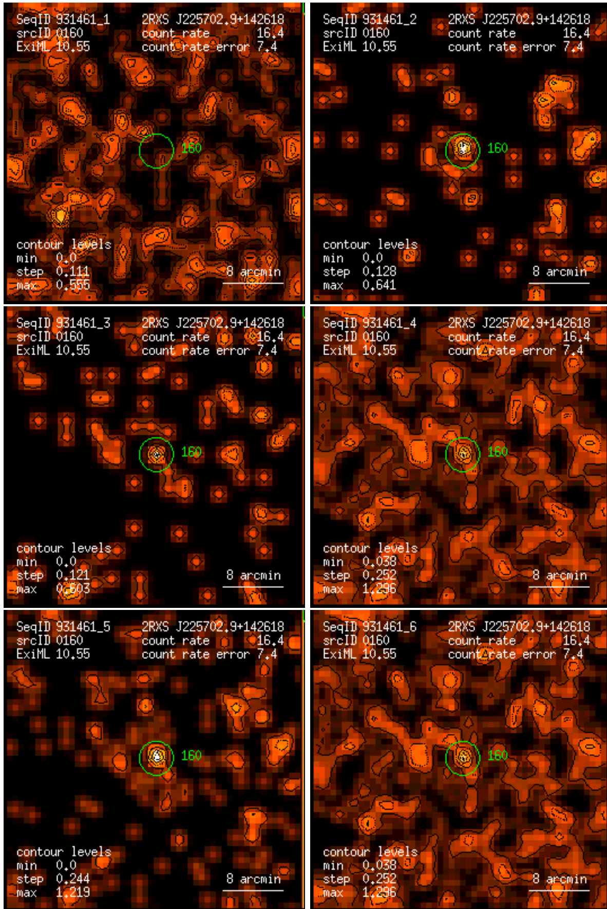
Figure 160: RASS 931461: detection 0160: band rate images, Gaussian filter: (1) PSPC channels 11 – 41, (2) 52 – 90, (3) 91 – 201, (4) 11 – 235, (5) 52 – 201, (6) 11 – 201. Broad band rates in counts/ks. Band rate contour levels in counts/ks/arcmin 2 .
