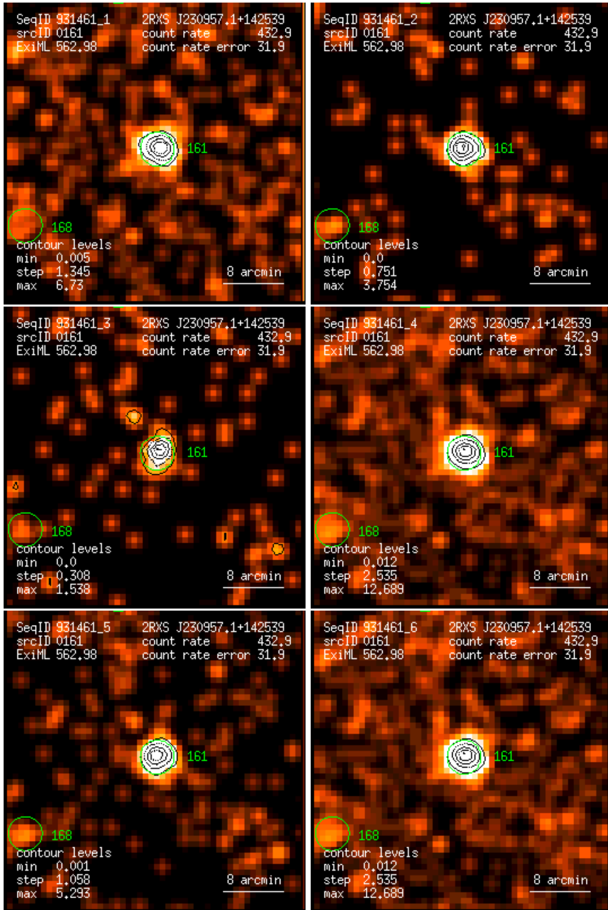
Figure 161: RASS 931461: detection 0161: band rate images, Gaussian filter: (1) PSPC channels 11 – 41, (2) 52 – 90, (3) 91 – 201, (4) 11 – 235, (5) 52 – 201, (6) 11 – 201. Broad band rates in counts/ks. Band rate contour levels in counts/ks/arcmin 2 .
