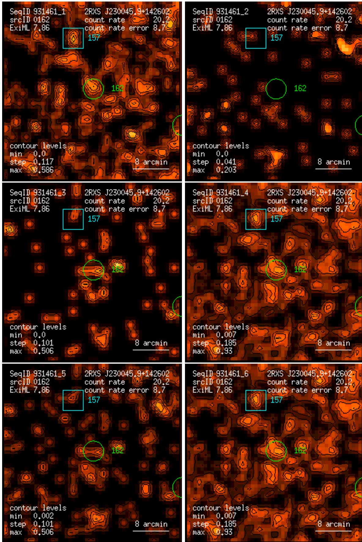
Figure 162: RASS 931461: detection 0162: band rate images, Gaussian filter: (1) PSPC channels 11 – 41, (2) 52 – 90, (3) 91 – 201, (4) 11 – 235, (5) 52 – 201, (6) 11 – 201. Broad band rates in counts/ks. Band rate contour levels in counts/ks/arcmin 2 .
