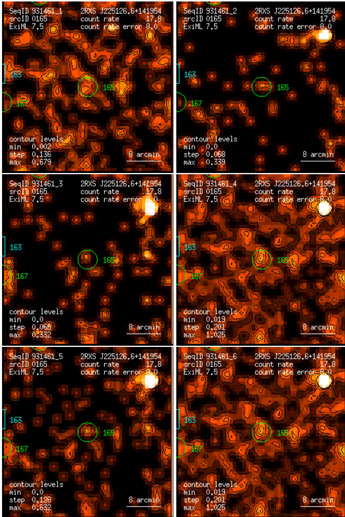
Figure 165: RASS 931461: detection 0165: band rate images, Gaussian filter: (1) PSPC channels 11 – 41, (2) 52 – 90, (3) 91 – 201, (4) 11 – 235, (5) 52 – 201, (6) 11 – 201. Broad band rates in counts/ks. Band rate contour levels in counts/ks/arcmin 2 .
