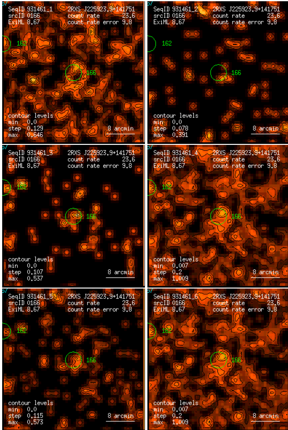
Figure 166: RASS 931461: detection 0166: band rate images, Gaussian filter: (1) PSPC channels 11 – 41, (2) 52 – 90, (3) 91 – 201, (4) 11 – 235, (5) 52 – 201, (6) 11 – 201. Broad band rates in counts/ks. Band rate contour levels in counts/ks/arcmin 2 .
