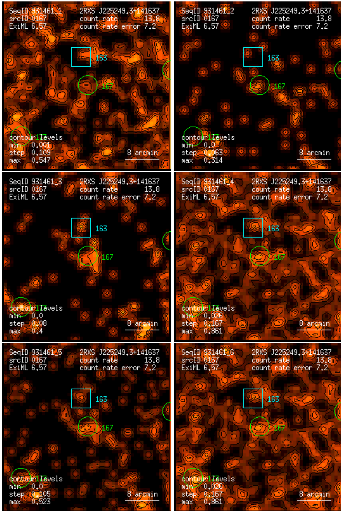
Figure 167: RASS 931461: detection 0167: band rate images, Gaussian filter: (1) PSPC channels 11 – 41, (2) 52 – 90, (3) 91 – 201, (4) 11 – 235, (5) 52 – 201, (6) 11 – 201. Broad band rates in counts/ks. Band rate contour levels in counts/ks/arcmin 2 .
