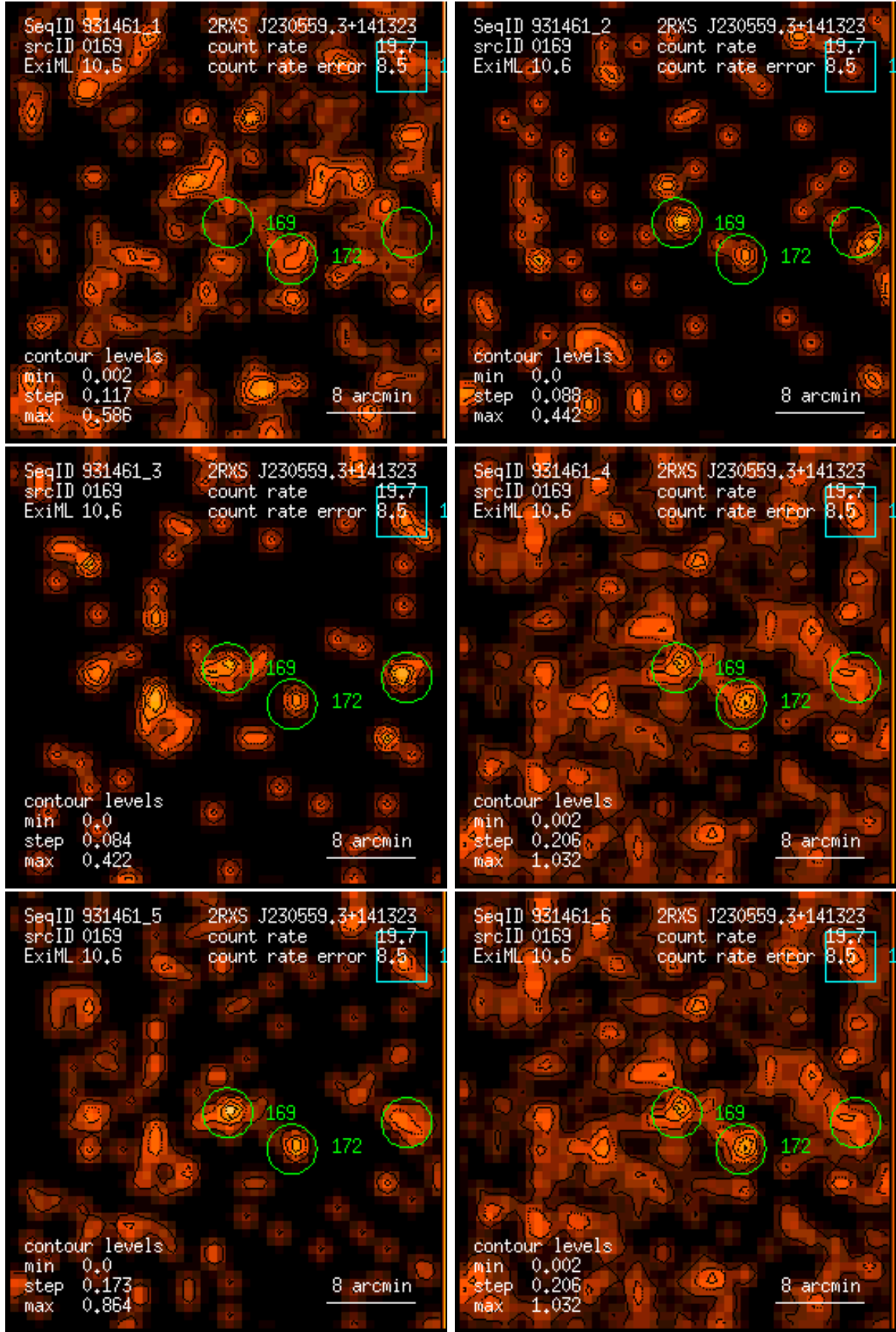
Figure 169: RASS 931461: detection 0169: band rate images, Gaussian filter: (1) PSPC channels 11 – 41, (2) 52 – 90, (3) 91 – 201, (4) 11 – 235, (5) 52 – 201, (6) 11 – 201. Broad band rates in counts/ks. Band rate contour levels in counts/ks/arcmin 2 .
