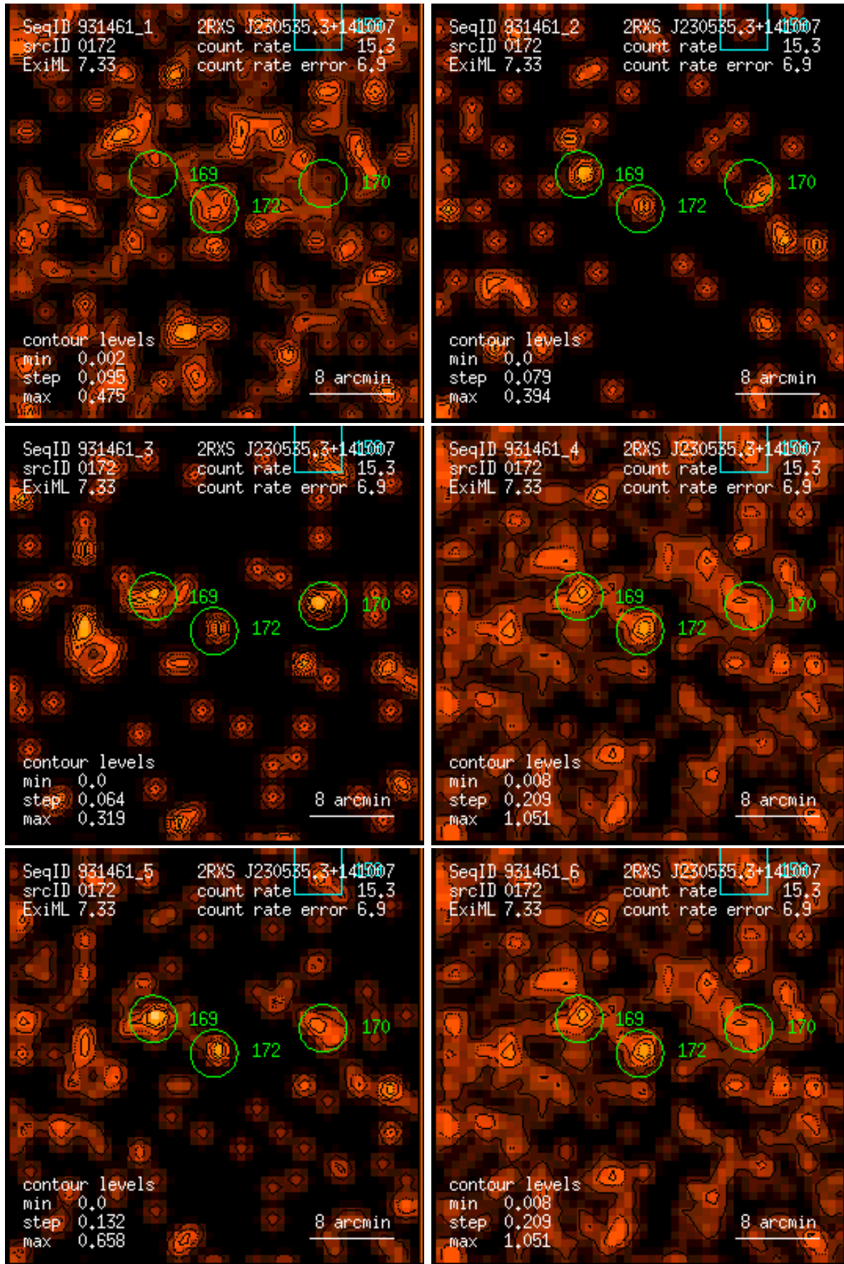
Figure 172: RASS 931461: detection 0172: band rate images, Gaussian filter: (1) PSPC channels 11 – 41, (2) 52 – 90, (3) 91 – 201, (4) 11 – 235, (5) 52 – 201, (6) 11 – 201. Broad band rates in counts/ks. Band rate contour levels in counts/ks/arcmin 2 .
