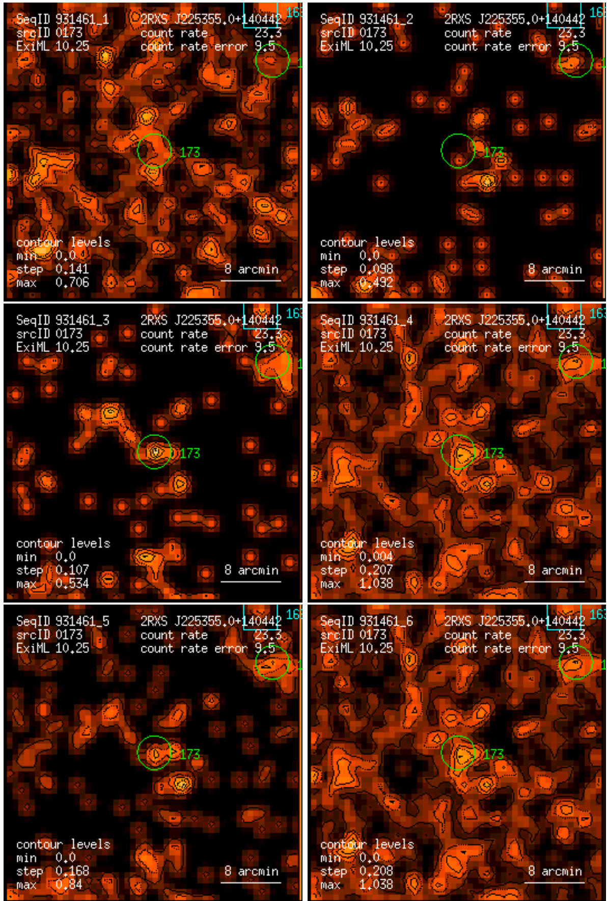
Figure 173: RASS 931461: detection 0173: band rate images, Gaussian filter: (1) PSPC channels 11 – 41, (2) 52 – 90, (3) 91 – 201, (4) 11 – 235, (5) 52 – 201, (6) 11 – 201. Broad band rates in counts/ks. Band rate contour levels in counts/ks/arcmin 2 .
