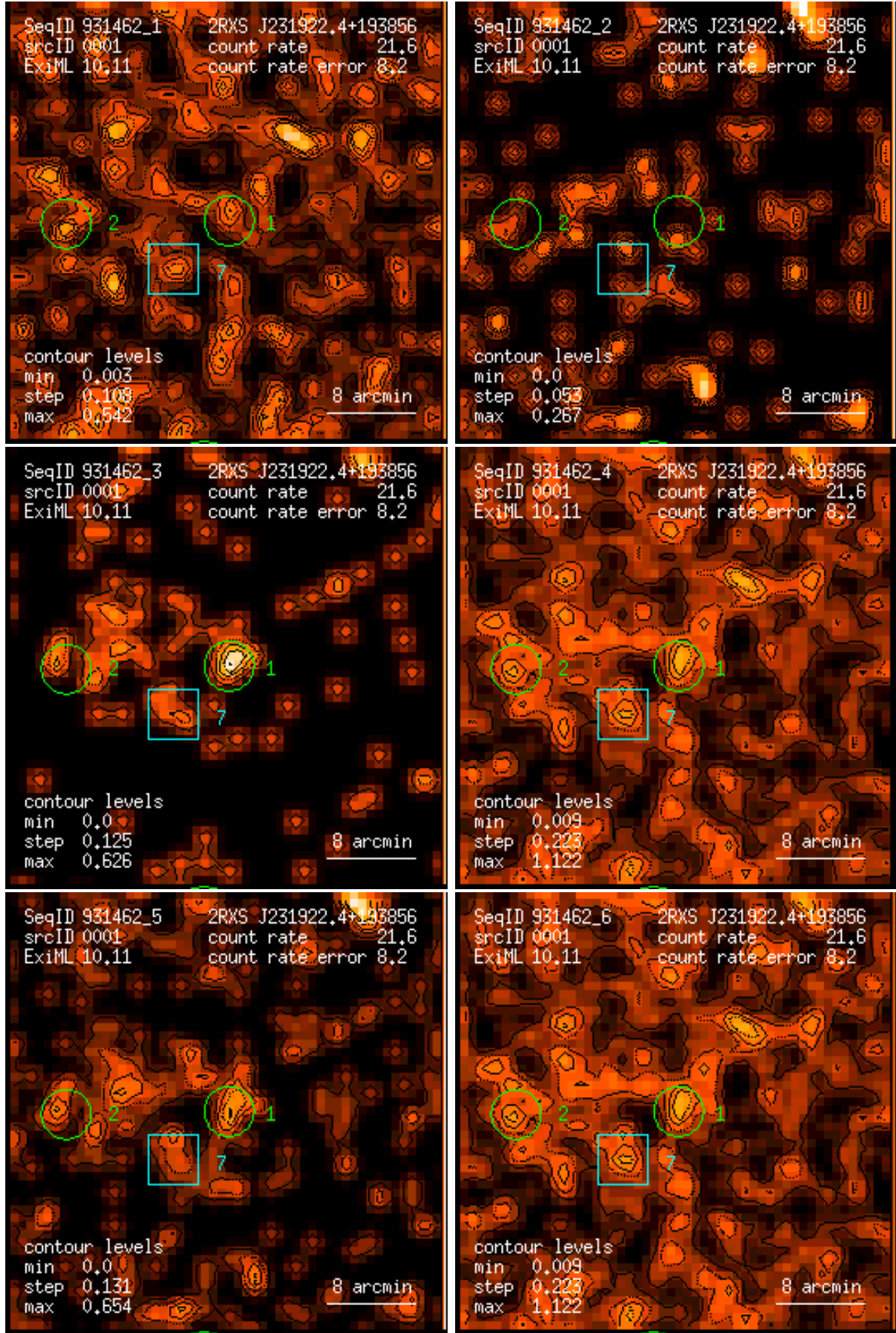
Figure 1: RASS 931462: detection 0001: band rate images, Gaussian filter: (1) PSPC channels 11 – 41, (2) 52 – 90, (3) 91 – 201, (4) 11 – 235, (5) 52 – 201, (6) 11 – 201. Broad band rates in counts/ks. Band rate contour levels in counts/ks/arcmin 2 .
