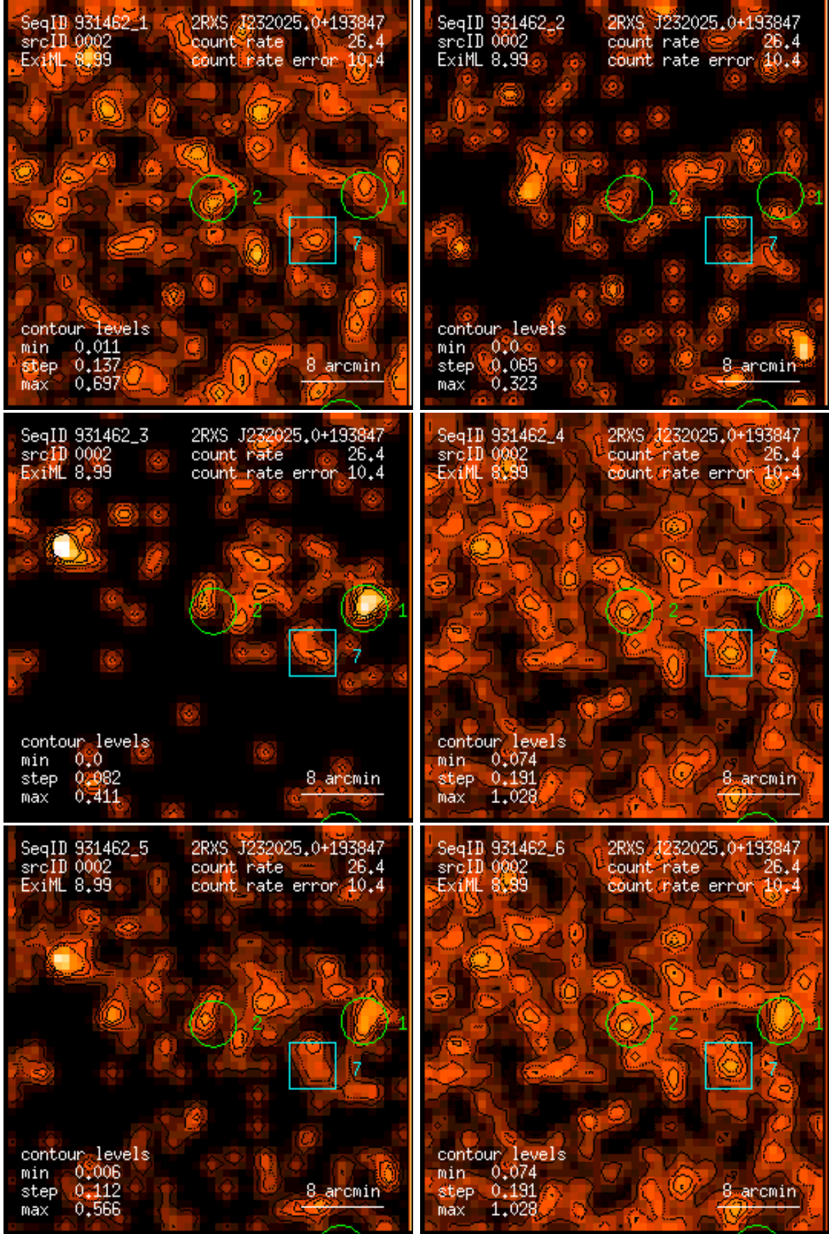
Figure 2: RASS 931462: detection 0002: band rate images, Gaussian filter: (1) PSPC channels 11 – 41, (2) 52 – 90, (3) 91 – 201, (4) 11 – 235, (5) 52 – 201, (6) 11 – 201. Broad band rates in counts/ks. Band rate contour levels in counts/ks/arcmin 2 .
