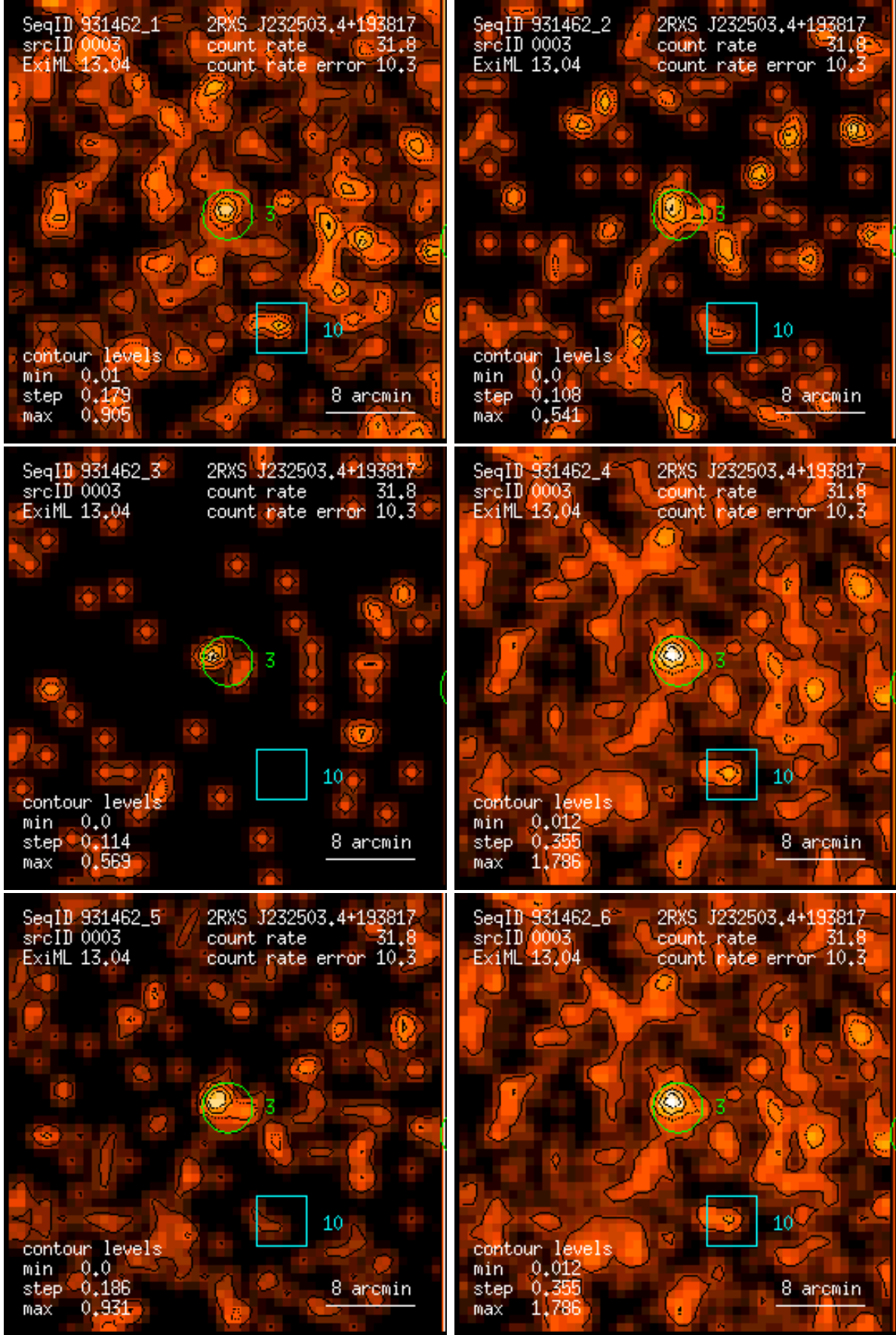
Figure 3: RASS 931462: detection 0003: band rate images, Gaussian filter: (1) PSPC channels 11 – 41, (2) 52 – 90, (3) 91 – 201, (4) 11 – 235, (5) 52 – 201, (6) 11 – 201. Broad band rates in counts/ks. Band rate contour levels in counts/ks/arcmin 2 .
