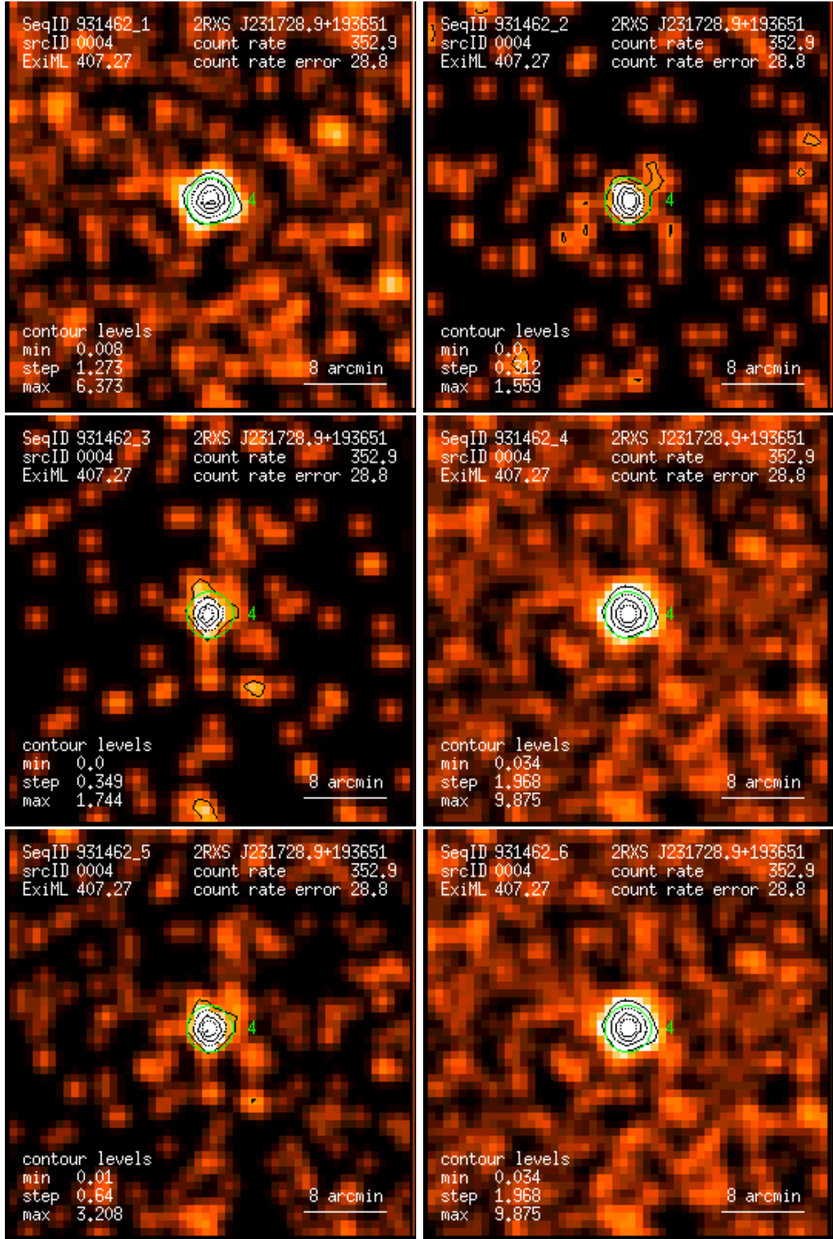
Figure 4: RASS 931462: detection 0004: band rate images, Gaussian filter: (1) PSPC channels 11 – 41, (2) 52 – 90, (3) 91 – 201, (4) 11 – 235, (5) 52 – 201, (6) 11 – 201. Broad band rates in counts/ks. Band rate contour levels in counts/ks/arcmin 2 .
