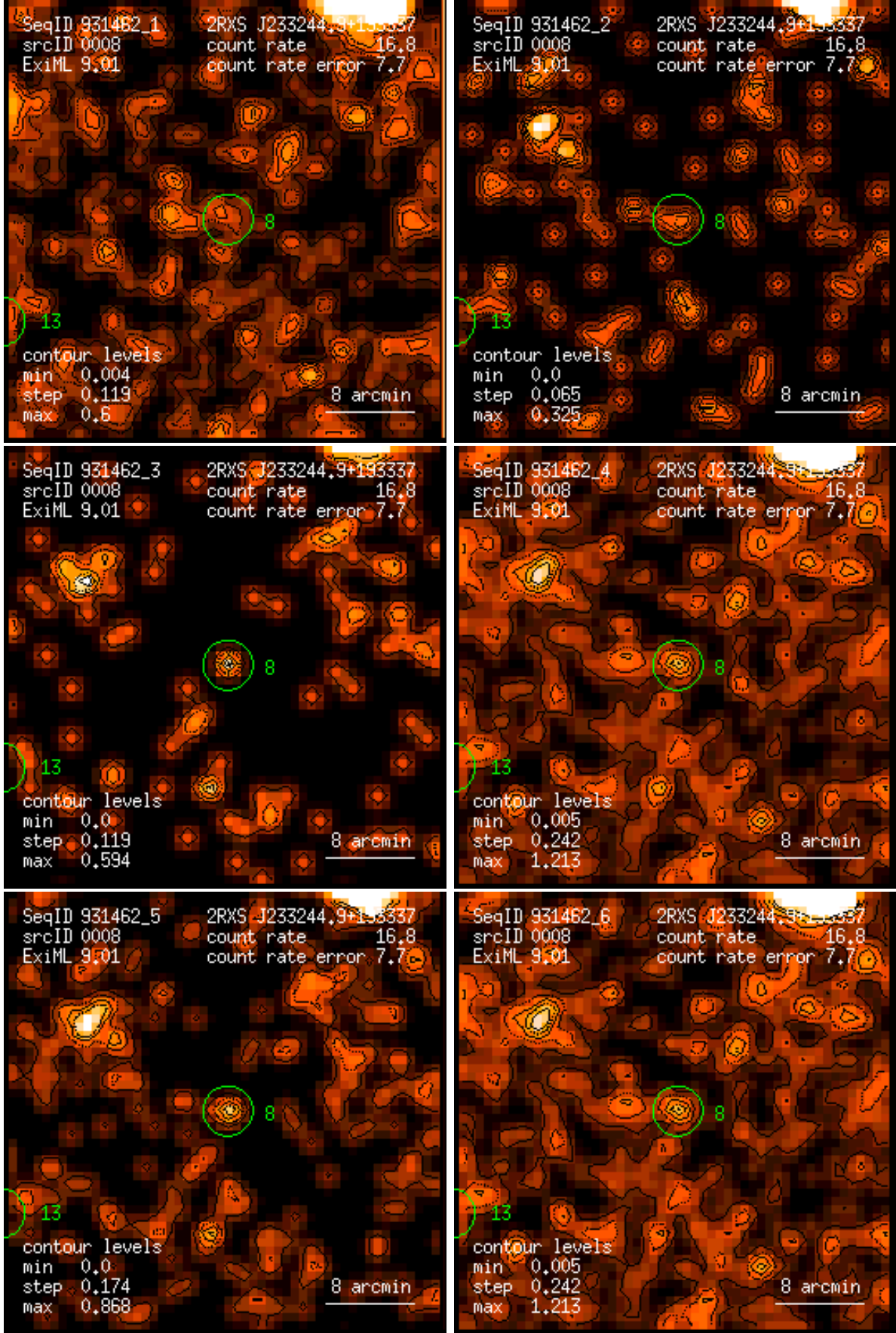
Figure 8: RASS 931462: detection 0008: band rate images, Gaussian filter: (1) PSPC channels 11 – 41, (2) 52 – 90, (3) 91 – 201, (4) 11 – 235, (5) 52 – 201, (6) 11 – 201. Broad band rates in counts/ks. Band rate contour levels in counts/ks/arcmin 2 .
