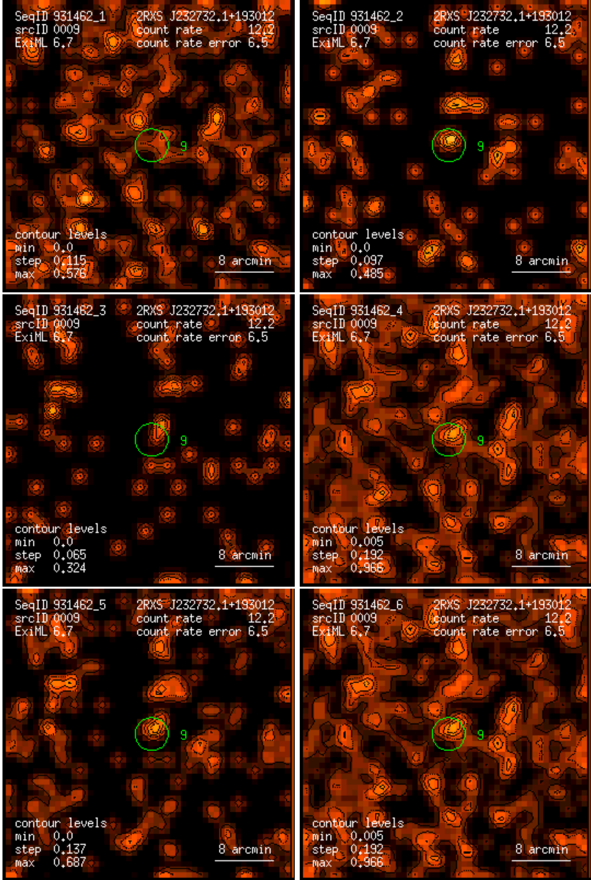
Figure 9: RASS 931462: detection 0009: band rate images, Gaussian filter: (1) PSPC channels 11 – 41, (2) 52 – 90, (3) 91 – 201, (4) 11 – 235, (5) 52 – 201, (6) 11 – 201. Broad band rates in counts/ks. Band rate contour levels in counts/ks/arcmin 2 .
