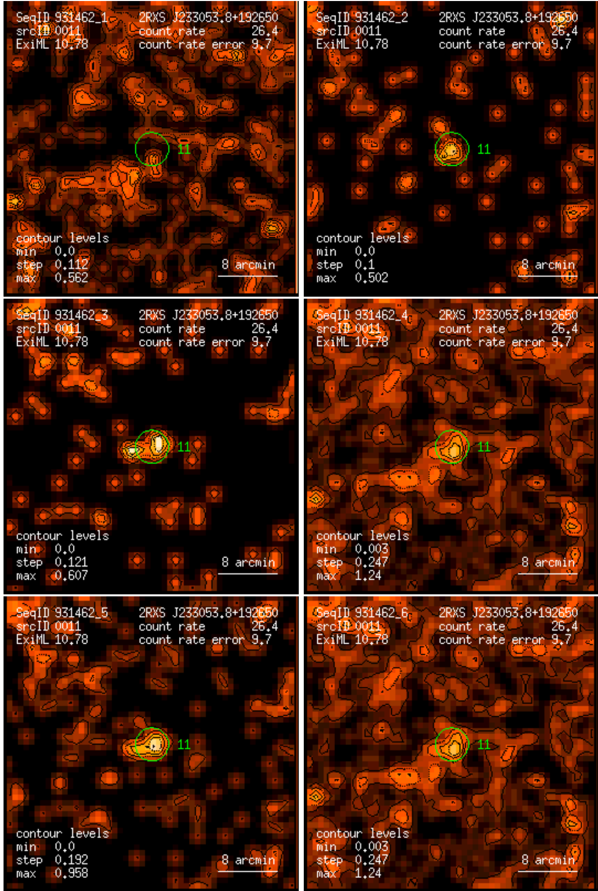
Figure 11: RASS 931462: detection 0011: band rate images, Gaussian filter: (1) PSPC channels 11 – 41, (2) 52 – 90, (3) 91 – 201, (4) 11 – 235, (5) 52 – 201, (6) 11 – 201. Broad band rates in counts/ks. Band rate contour levels in counts/ks/arcmin 2 .
