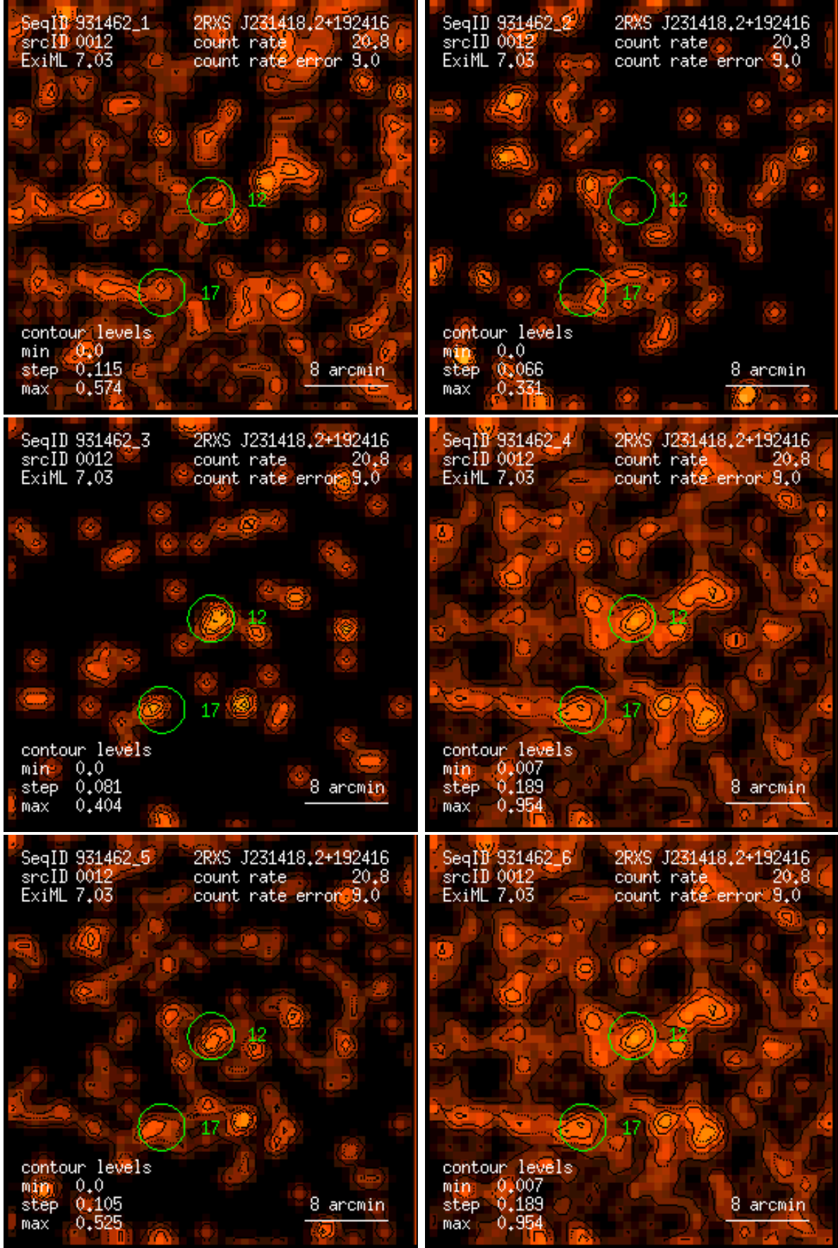
Figure 12: RASS 931462: detection 0012: band rate images, Gaussian filter: (1) PSPC channels 11 – 41, (2) 52 – 90, (3) 91 – 201, (4) 11 – 235, (5) 52 – 201, (6) 11 – 201. Broad band rates in counts/ks. Band rate contour levels in counts/ks/arcmin 2 .
