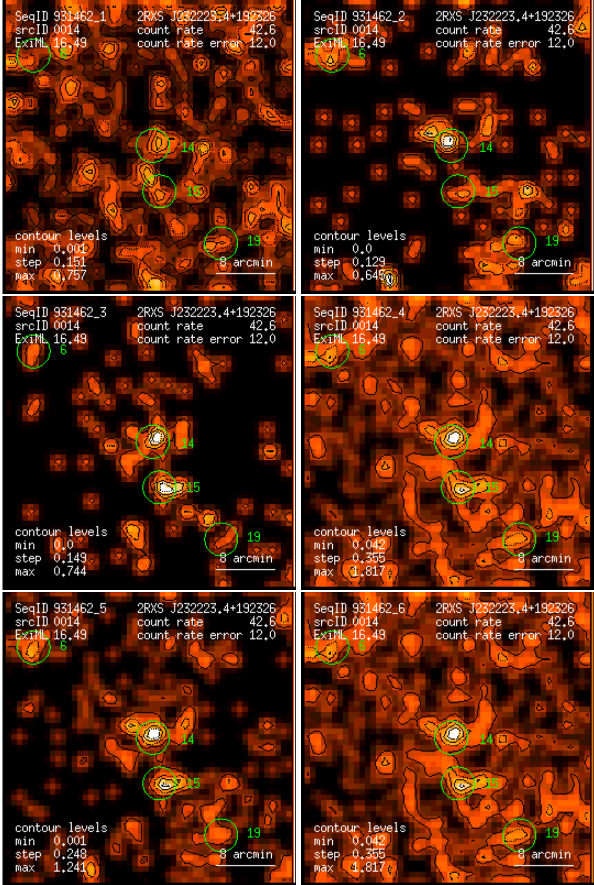
Figure 14: RASS 931462: detection 0014: band rate images, Gaussian filter: (1) PSPC channels 11 – 41, (2) 52 – 90, (3) 91 – 201, (4) 11 – 235, (5) 52 – 201, (6) 11 – 201. Broad band rates in counts/ks. Band rate contour levels in counts/ks/arcmin 2 .
