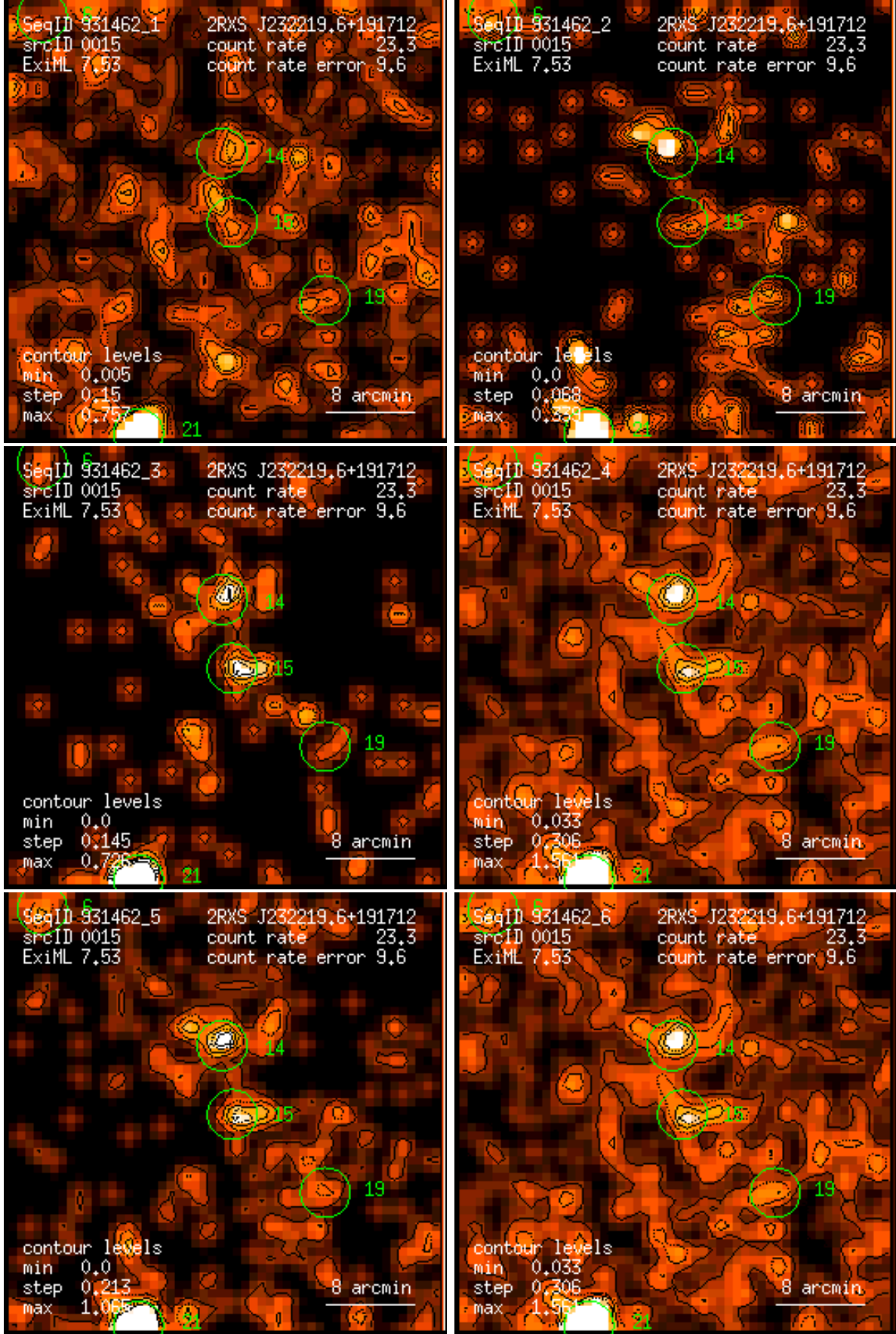
Figure 15: RASS 931462: detection 0015: band rate images, Gaussian filter: (1) PSPC channels 11 – 41, (2) 52 – 90, (3) 91 – 201, (4) 11 – 235, (5) 52 – 201, (6) 11 – 201. Broad band rates in counts/ks. Band rate contour levels in counts/ks/arcmin 2 .
