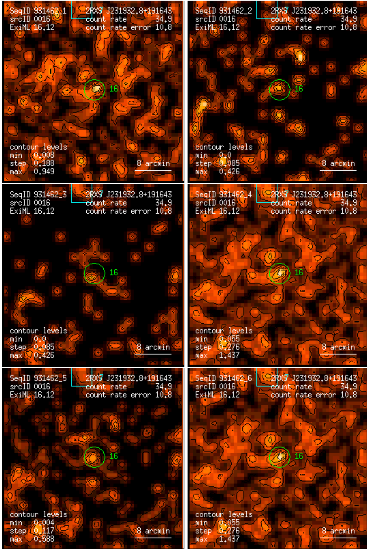
Figure 16: RASS 931462: detection 0016: band rate images, Gaussian filter: (1) PSPC channels 11 – 41, (2) 52 – 90, (3) 91 – 201, (4) 11 – 235, (5) 52 – 201, (6) 11 – 201. Broad band rates in counts/ks. Band rate contour levels in counts/ks/arcmin 2 .
