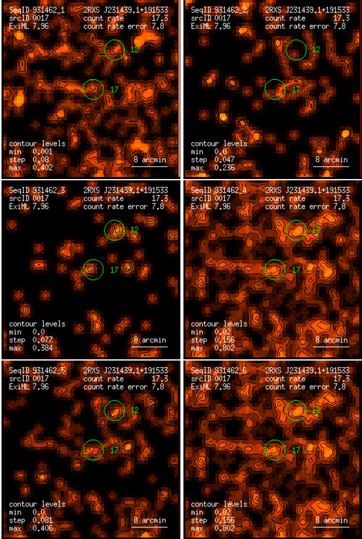
Figure 17: RASS 931462: detection 0017: band rate images, Gaussian filter: (1) PSPC channels 11 – 41, (2) 52 – 90, (3) 91 – 201, (4) 11 – 235, (5) 52 – 201, (6) 11 – 201. Broad band rates in counts/ks. Band rate contour levels in counts/ks/arcmin 2 .
