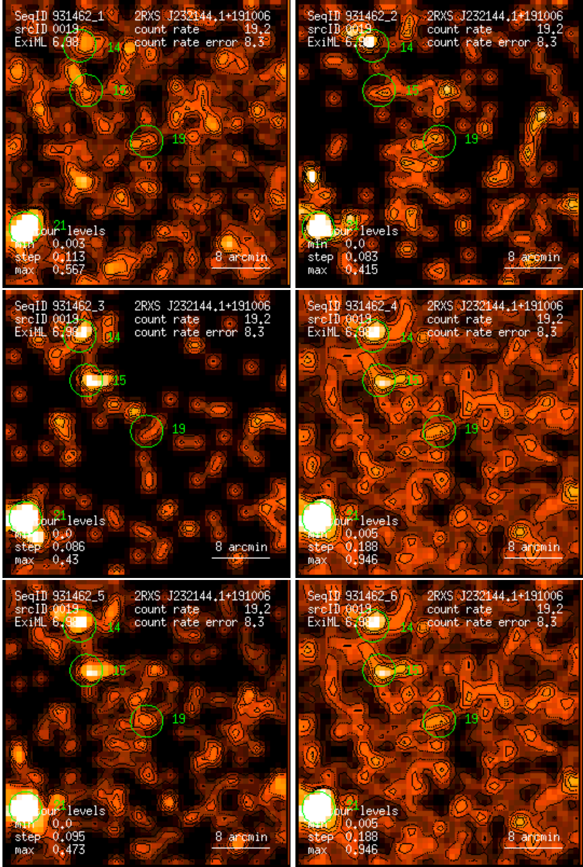
Figure 19: RASS 931462: detection 0019: band rate images, Gaussian filter: (1) PSPC channels 11 – 41, (2) 52 – 90, (3) 91 – 201, (4) 11 – 235, (5) 52 – 201, (6) 11 – 201. Broad band rates in counts/ks. Band rate contour levels in counts/ks/arcmin 2 .
