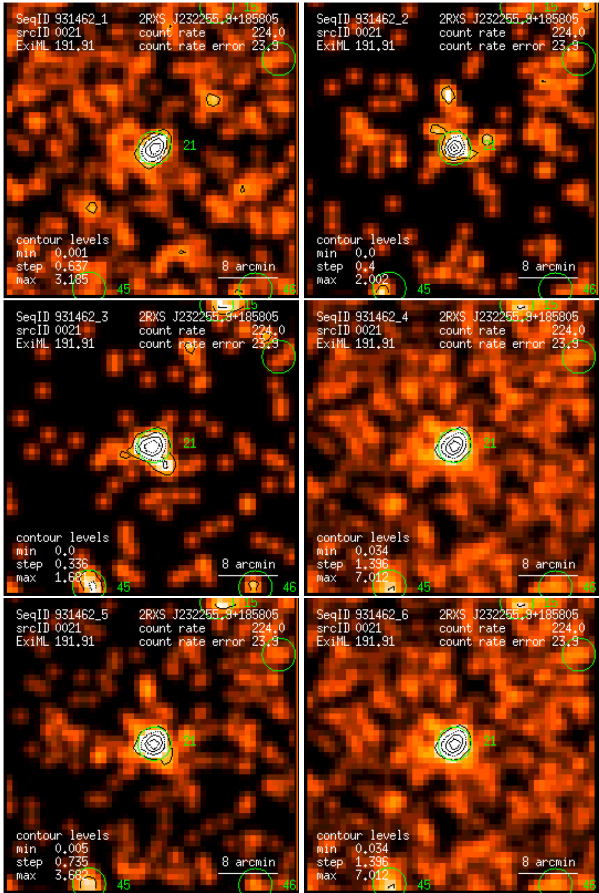
Figure 21: RASS 931462: detection 0021: band rate images, Gaussian filter: (1) PSPC channels 11 – 41, (2) 52 – 90, (3) 91 – 201, (4) 11 – 235, (5) 52 – 201, (6) 11 – 201. Broad band rates in counts/ks. Band rate contour levels in counts/ks/arcmin 2 .
