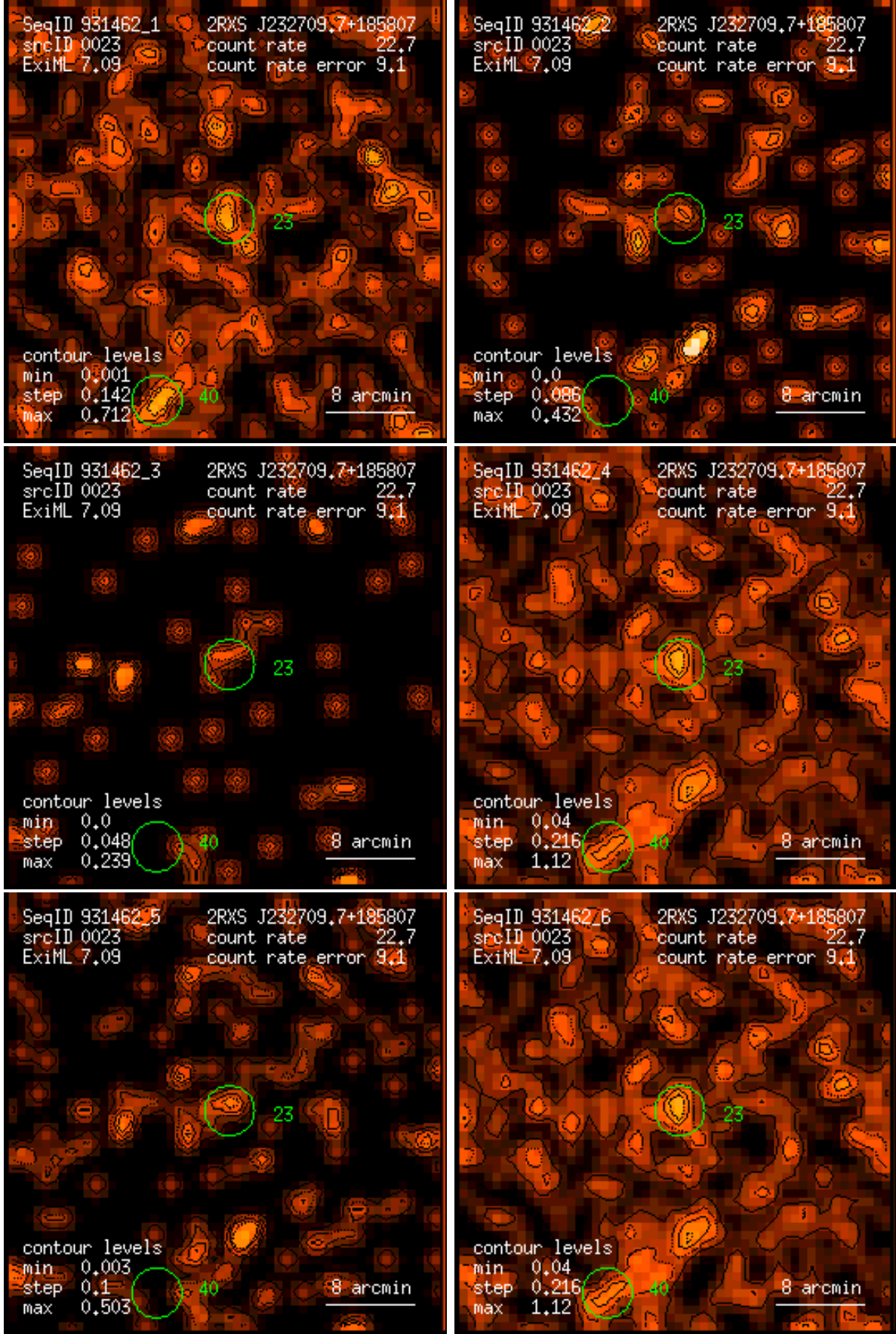
Figure 23: RASS 931462: detection 0023: band rate images, Gaussian filter: (1) PSPC channels 11 – 41, (2) 52 – 90, (3) 91 – 201, (4) 11 – 235, (5) 52 – 201, (6) 11 – 201. Broad band rates in counts/ks. Band rate contour levels in counts/ks/arcmin 2 .
