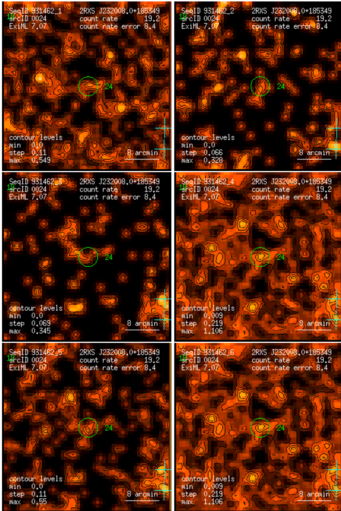
Figure 24: RASS 931462: detection 0024: band rate images, Gaussian filter: (1) PSPC channels 11 – 41, (2) 52 – 90, (3) 91 – 201, (4) 11 – 235, (5) 52 – 201, (6) 11 – 201. Broad band rates in counts/ks. Band rate contour levels in counts/ks/arcmin 2 .
