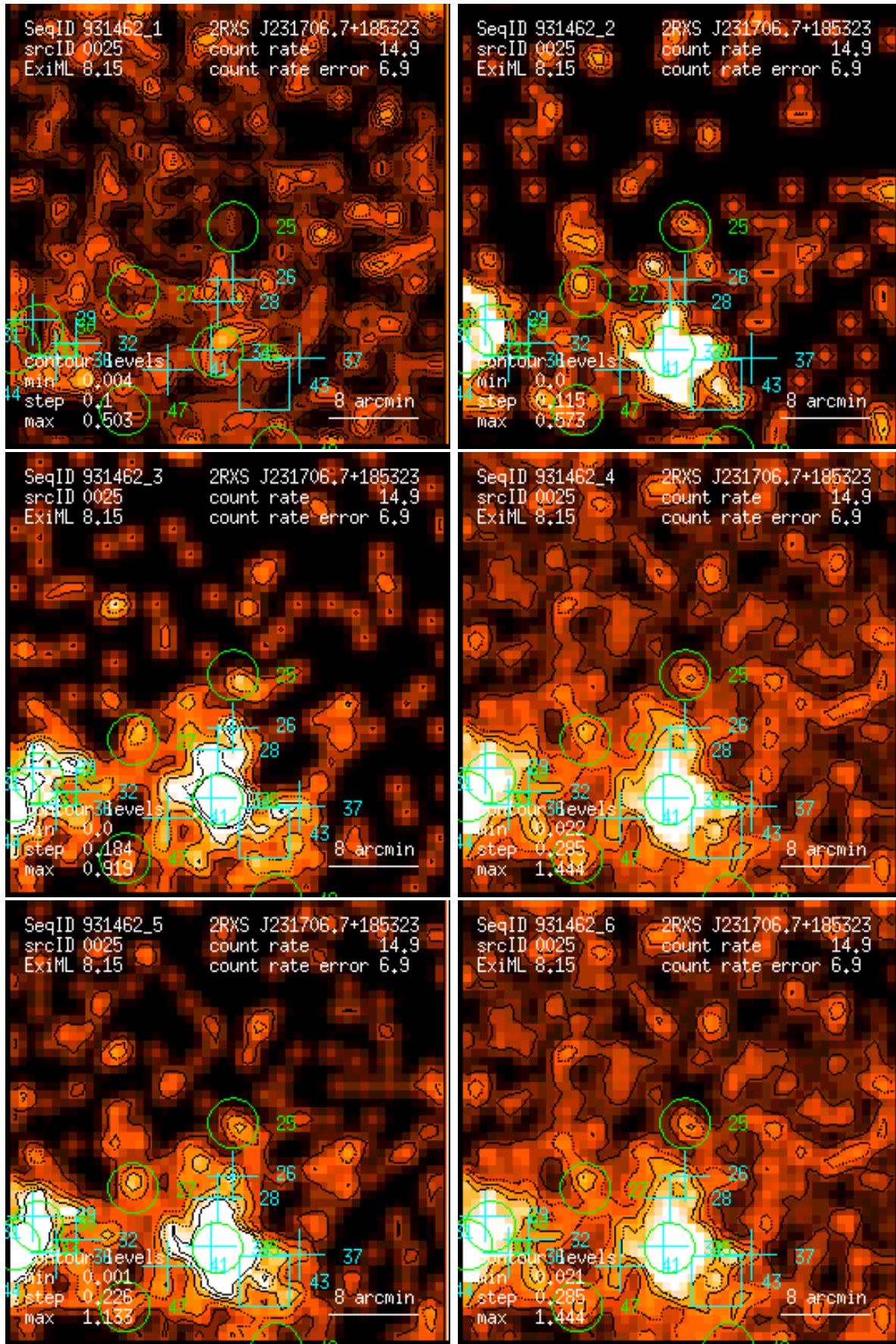
Figure 25: RASS 931462: detection 0025: band rate images, Gaussian filter: (1) PSPC channels 11 – 41, (2) 52 – 90, (3) 91 – 201, (4) 11 – 235, (5) 52 – 201, (6) 11 – 201. Broad band rates in counts/ks. Band rate contour levels in counts/ks/arcmin 2 .
