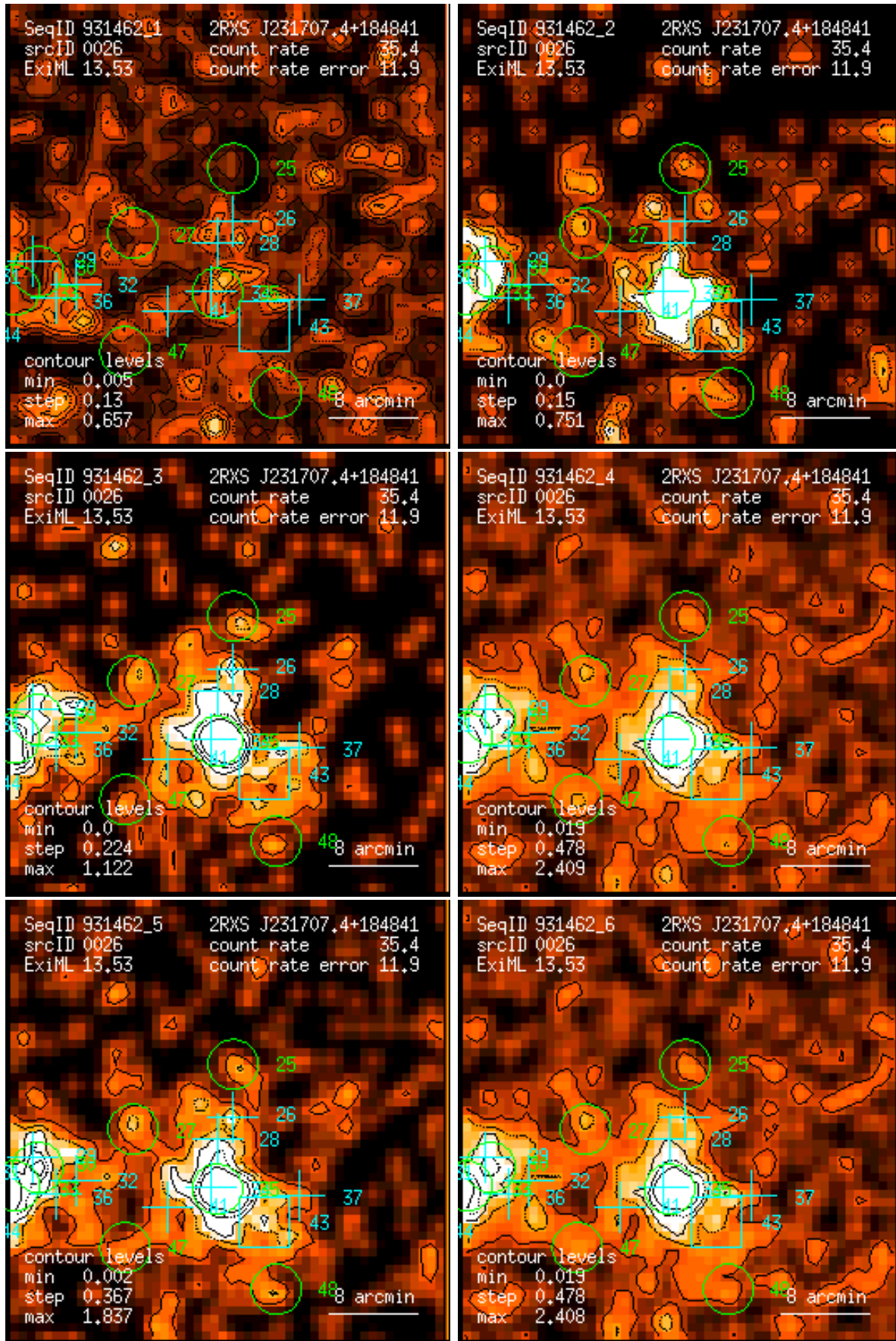
Figure 26: RASS 931462: detection 0026: band rate images, Gaussian filter: (1) PSPC channels 11 – 41, (2) 52 – 90, (3) 91 – 201, (4) 11 – 235, (5) 52 – 201, (6) 11 – 201. Broad band rates in counts/ks. Band rate contour levels in counts/ks/arcmin 2 .
