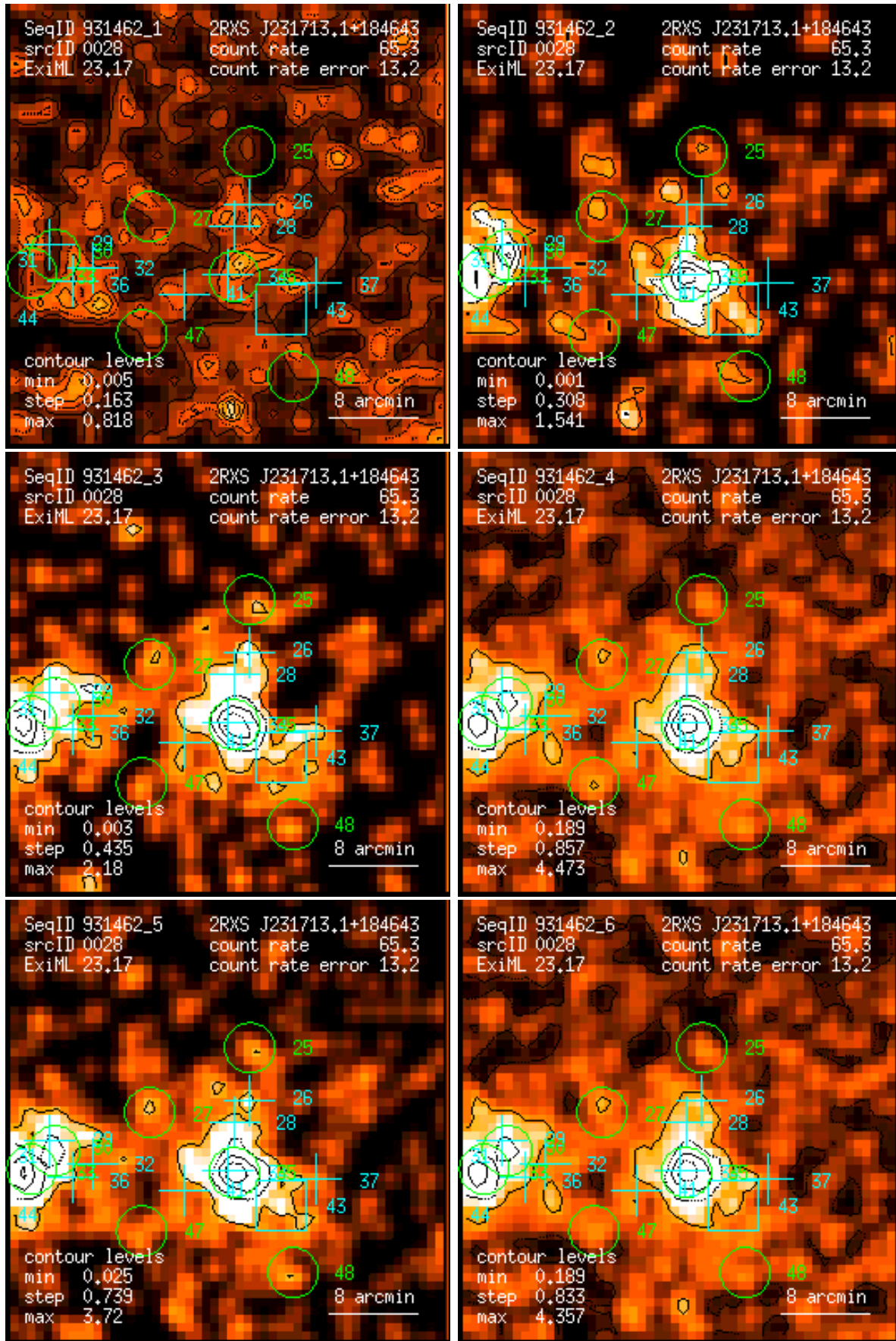
Figure 28: RASS 931462: detection 0028: band rate images, Gaussian filter: (1) PSPC channels 11 – 41, (2) 52 – 90, (3) 91 – 201, (4) 11 – 235, (5) 52 – 201, (6) 11 – 201. Broad band rates in counts/ks. Band rate contour levels in counts/ks/arcmin 2 .
