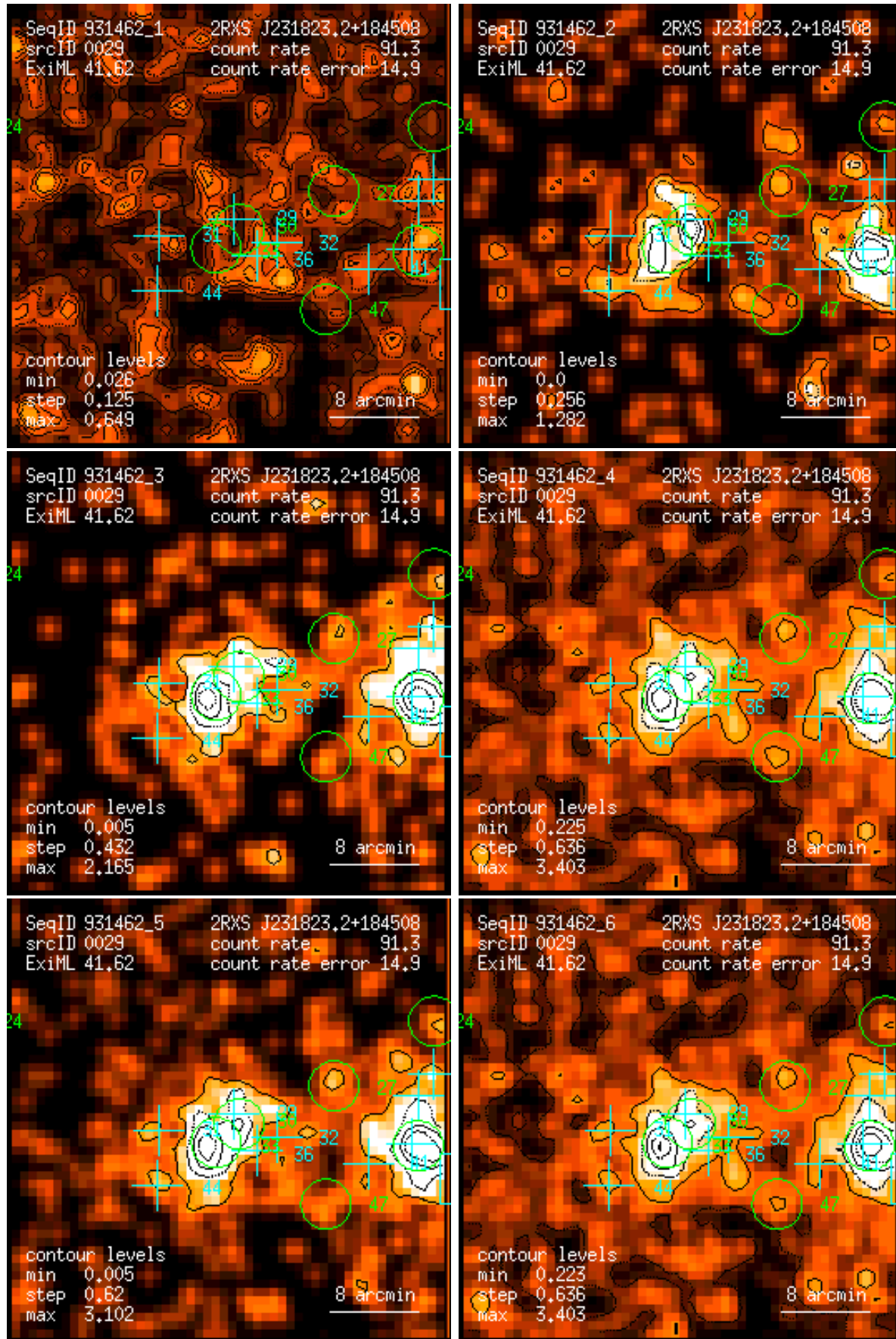
Figure 29: RASS 931462: detection 0029: band rate images, Gaussian filter: (1) PSPC channels 11 – 41, (2) 52 – 90, (3) 91 – 201, (4) 11 – 235, (5) 52 – 201, (6) 11 – 201. Broad band rates in counts/ks. Band rate contour levels in counts/ks/arcmin 2 .
