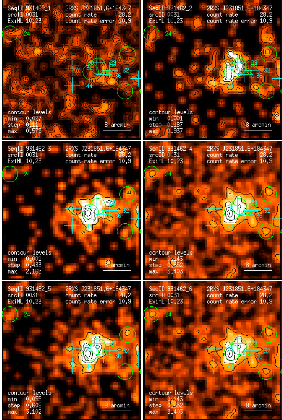
Figure 31: RASS 931462: detection 0031: band rate images, Gaussian filter: (1) PSPC channels 11 – 41, (2) 52 – 90, (3) 91 – 201, (4) 11 – 235, (5) 52 – 201, (6) 11 – 201. Broad band rates in counts/ks. Band rate contour levels in counts/ks/arcmin 2 .
