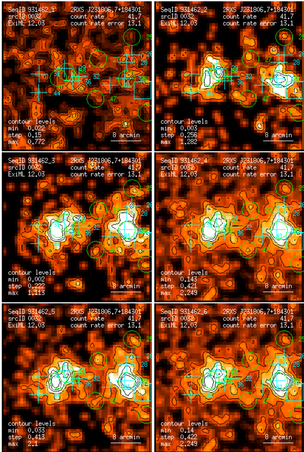
Figure 32: RASS 931462: detection 0032: band rate images, Gaussian filter: (1) PSPC channels 11 – 41, (2) 52 – 90, (3) 91 – 201, (4) 11 – 235, (5) 52 – 201, (6) 11 – 201. Broad band rates in counts/ks. Band rate contour levels in counts/ks/arcmin 2 .
