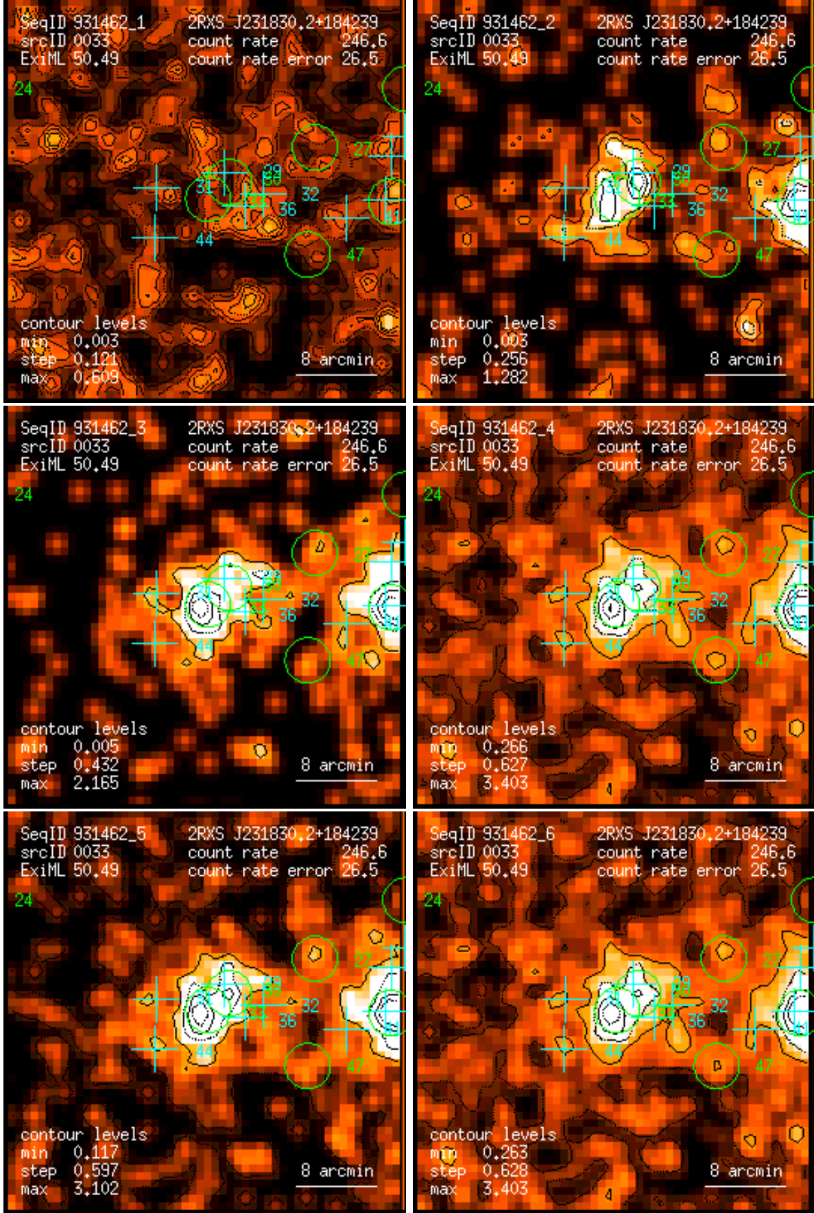
Figure 33: RASS 931462: detection 0033: band rate images, Gaussian filter: (1) PSPC channels 11 – 41, (2) 52 – 90, (3) 91 – 201, (4) 11 – 235, (5) 52 – 201, (6) 11 – 201. Broad band rates in counts/ks. Band rate contour levels in counts/ks/arcmin 2 .
