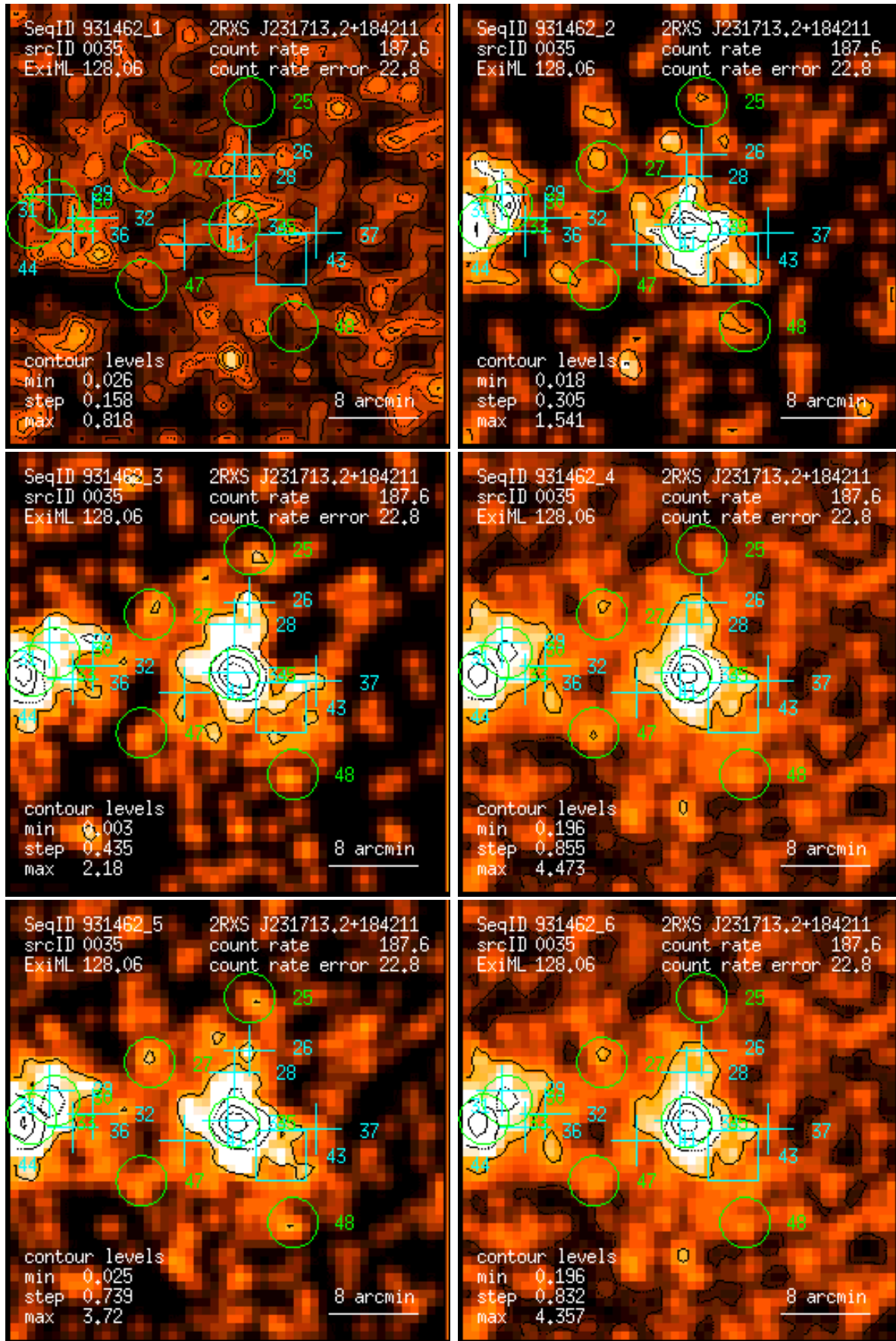
Figure 35: RASS 931462: detection 0035: band rate images, Gaussian filter: (1) PSPC channels 11 – 41, (2) 52 – 90, (3) 91 – 201, (4) 11 – 235, (5) 52 – 201, (6) 11 – 201. Broad band rates in counts/ks. Band rate contour levels in counts/ks/arcmin 2 .
