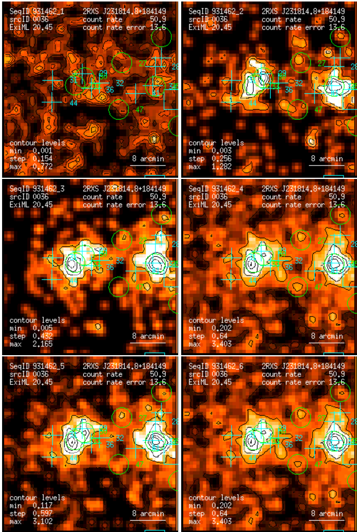
Figure 36: RASS 931462: detection 0036: band rate images, Gaussian filter: (1) PSPC channels 11 – 41, (2) 52 – 90, (3) 91 – 201, (4) 11 – 235, (5) 52 – 201, (6) 11 – 201. Broad band rates in counts/ks. Band rate contour levels in counts/ks/arcmin 2 .
