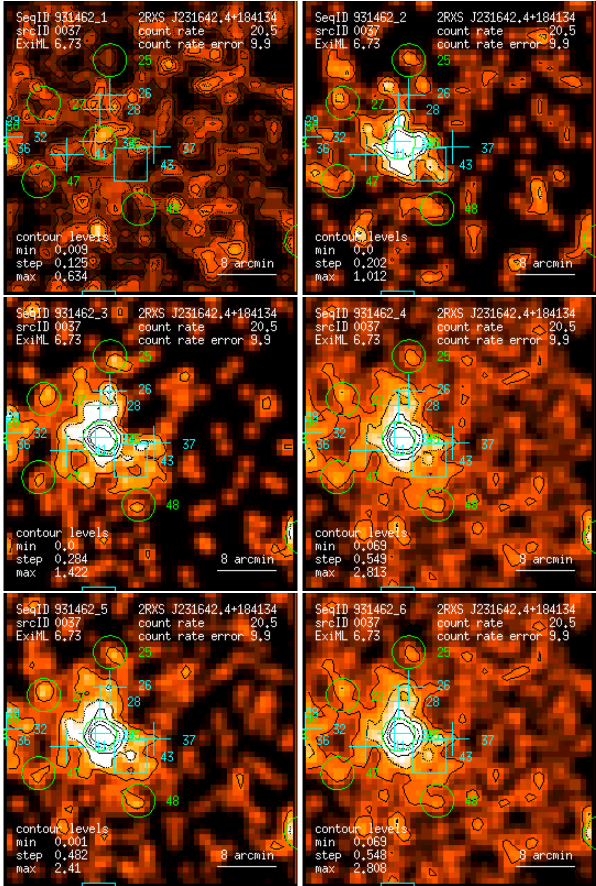
Figure 37: RASS 931462: detection 0037: band rate images, Gaussian filter: (1) PSPC channels 11 – 41, (2) 52 – 90, (3) 91 – 201, (4) 11 – 235, (5) 52 – 201, (6) 11 – 201. Broad band rates in counts/ks. Band rate contour levels in counts/ks/arcmin 2 .
