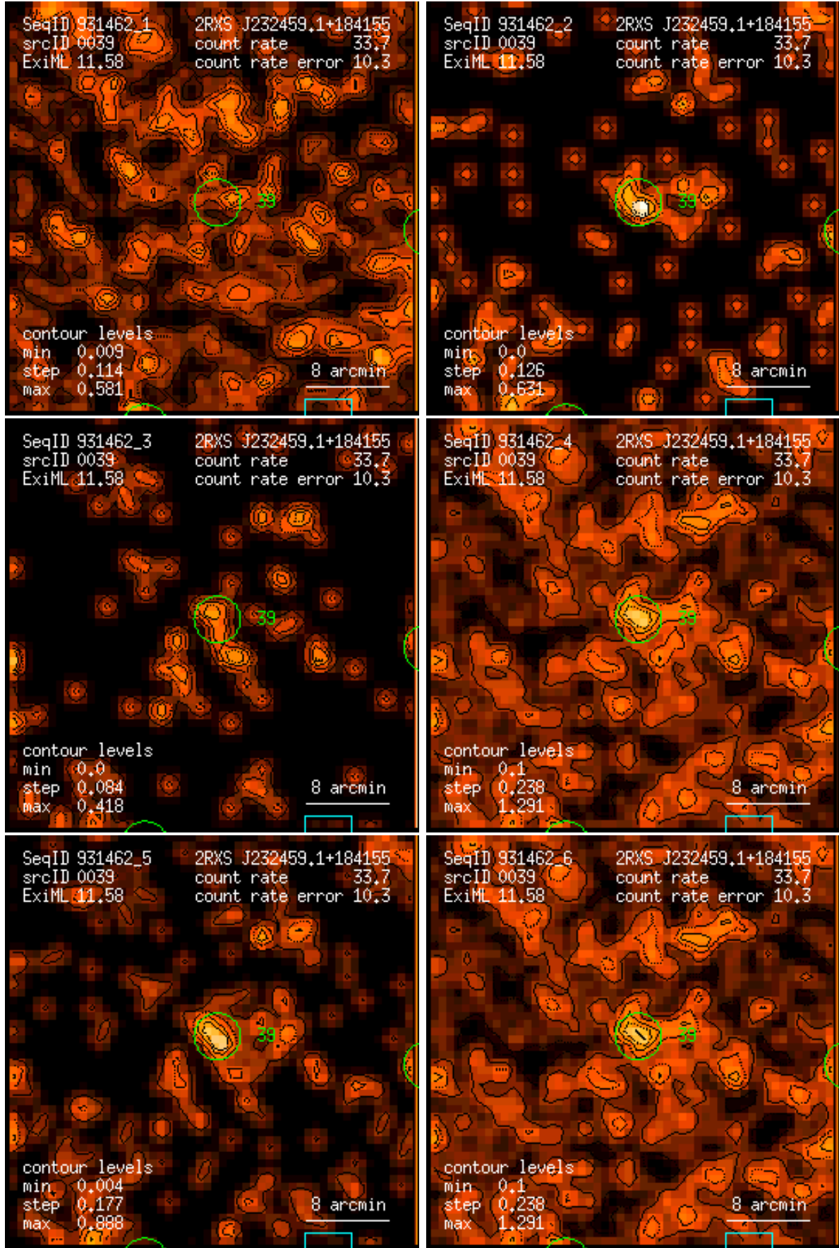
Figure 39: RASS 931462: detection 0039: band rate images, Gaussian filter: (1) PSPC channels 11 – 41, (2) 52 – 90, (3) 91 – 201, (4) 11 – 235, (5) 52 – 201, (6) 11 – 201. Broad band rates in counts/ks. Band rate contour levels in counts/ks/arcmin 2 .
