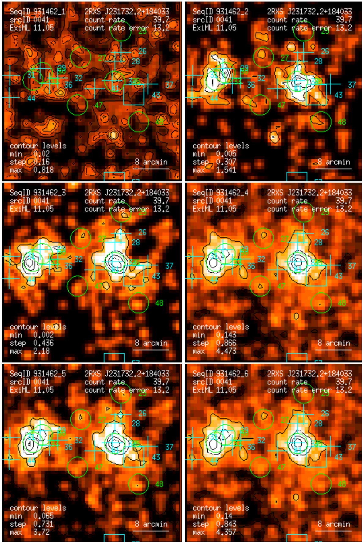
Figure 41: RASS 931462: detection 0041: band rate images, Gaussian filter: (1) PSPC channels 11 – 41, (2) 52 – 90, (3) 91 – 201, (4) 11 – 235, (5) 52 – 201, (6) 11 – 201. Broad band rates in counts/ks. Band rate contour levels in counts/ks/arcmin 2 .
