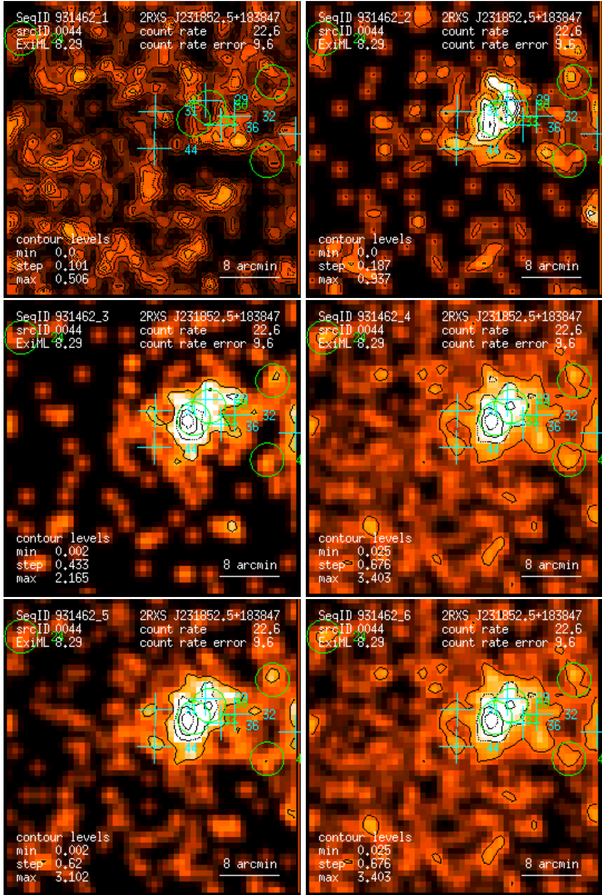
Figure 44: RASS 931462: detection 0044: band rate images, Gaussian filter: (1) PSPC channels 11 – 41, (2) 52 – 90, (3) 91 – 201, (4) 11 – 235, (5) 52 – 201, (6) 11 – 201. Broad band rates in counts/ks. Band rate contour levels in counts/ks/arcmin 2 .
