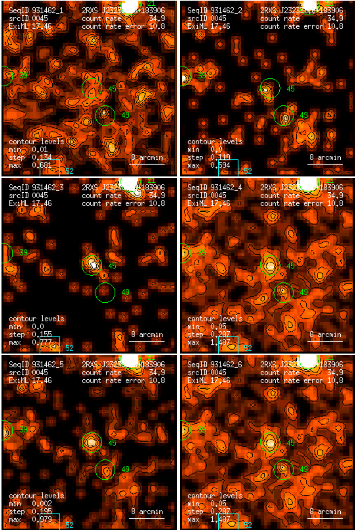
Figure 45: RASS 931462: detection 0045: band rate images, Gaussian filter: (1) PSPC channels 11 – 41, (2) 52 – 90, (3) 91 – 201, (4) 11 – 235, (5) 52 – 201, (6) 11 – 201. Broad band rates in counts/ks. Band rate contour levels in counts/ks/arcmin 2 .
