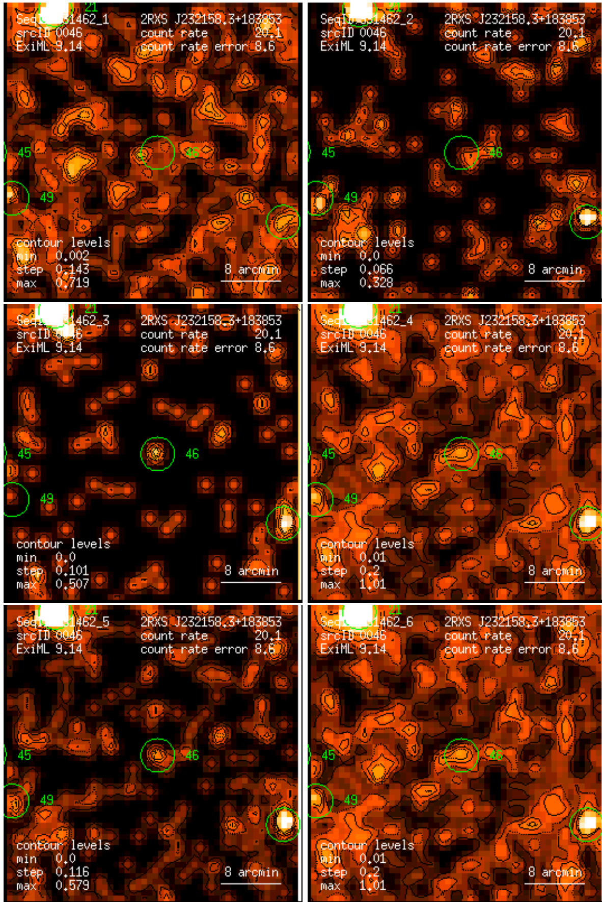
Figure 46: RASS 931462: detection 0046: band rate images, Gaussian filter: (1) PSPC channels 11 – 41, (2) 52 – 90, (3) 91 – 201, (4) 11 – 235, (5) 52 – 201, (6) 11 – 201. Broad band rates in counts/ks. Band rate contour levels in counts/ks/arcmin 2 .
